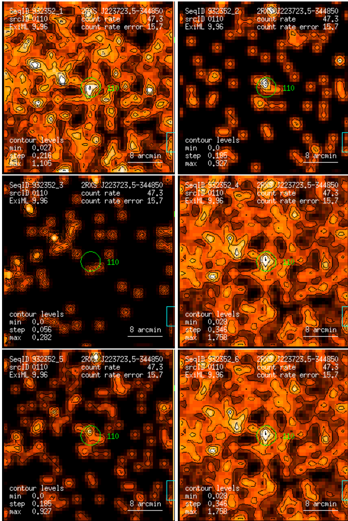
Figure 110: RASS 932352: detection 0110: band rate images, Gaussian filter: (1) PSPC channels 11 – 41, (2) 52 – 90, (3) 91 – 201, (4) 11 – 235, (5) 52 – 201, (6) 11 – 201. Broad band rates in counts/ks. Band rate contour levels in counts/ks/arcmin 2 .
