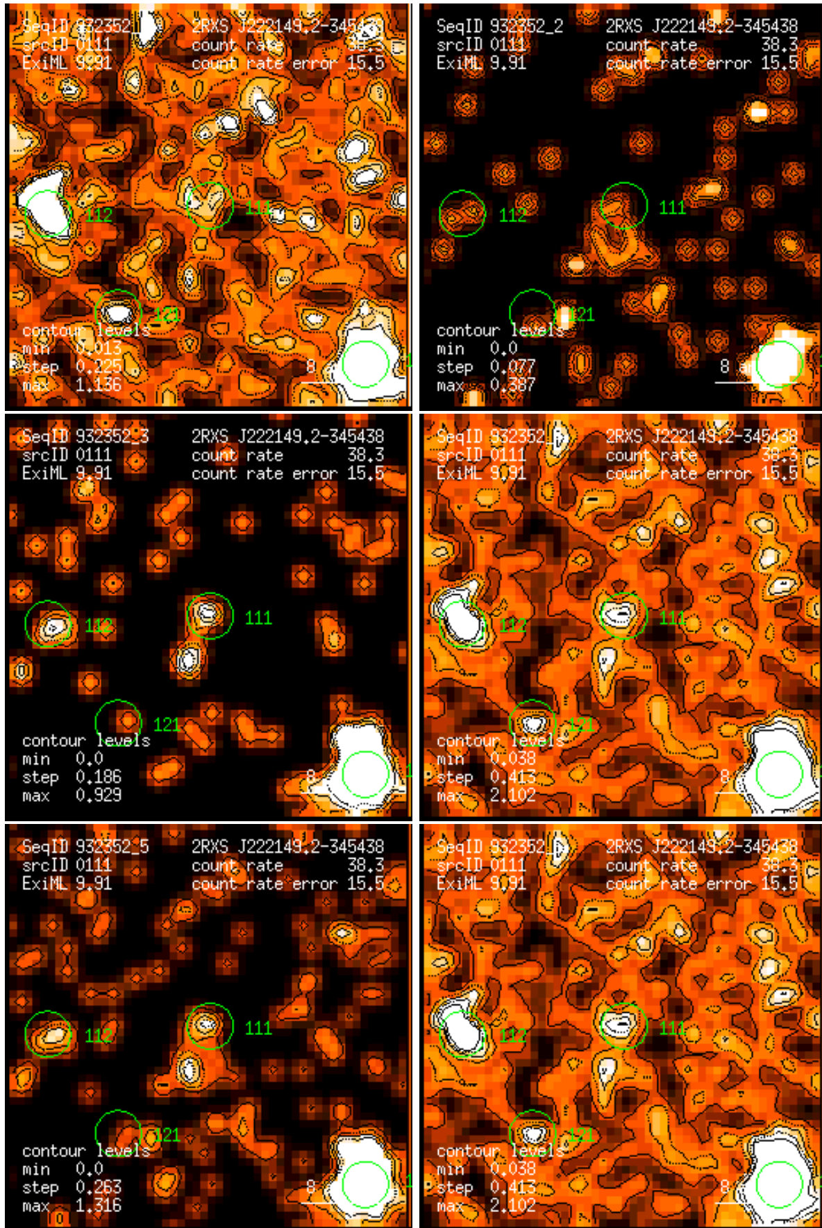
Figure 111: RASS 932352: detection 0111: band rate images, Gaussian filter: (1) PSPC channels 11 – 41, (2) 52 – 90, (3) 91 – 201, (4) 11 – 235, (5) 52 – 201, (6) 11 – 201. Broad band rates in counts/ks. Band rate contour levels in counts/ks/arcmin 2 .
