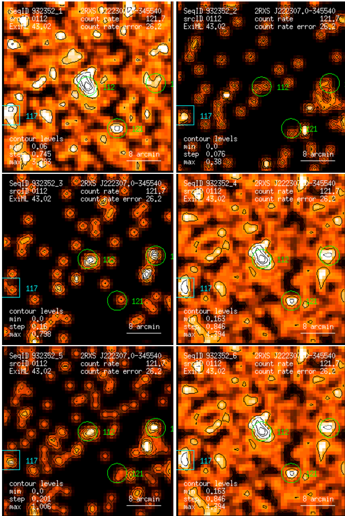
Figure 112: RASS 932352: detection 0112: band rate images, Gaussian filter: (1) PSPC channels 11 – 41, (2) 52 – 90, (3) 91 – 201, (4) 11 – 235, (5) 52 – 201, (6) 11 – 201. Broad band rates in counts/ks. Band rate contour levels in counts/ks/arcmin 2 .
