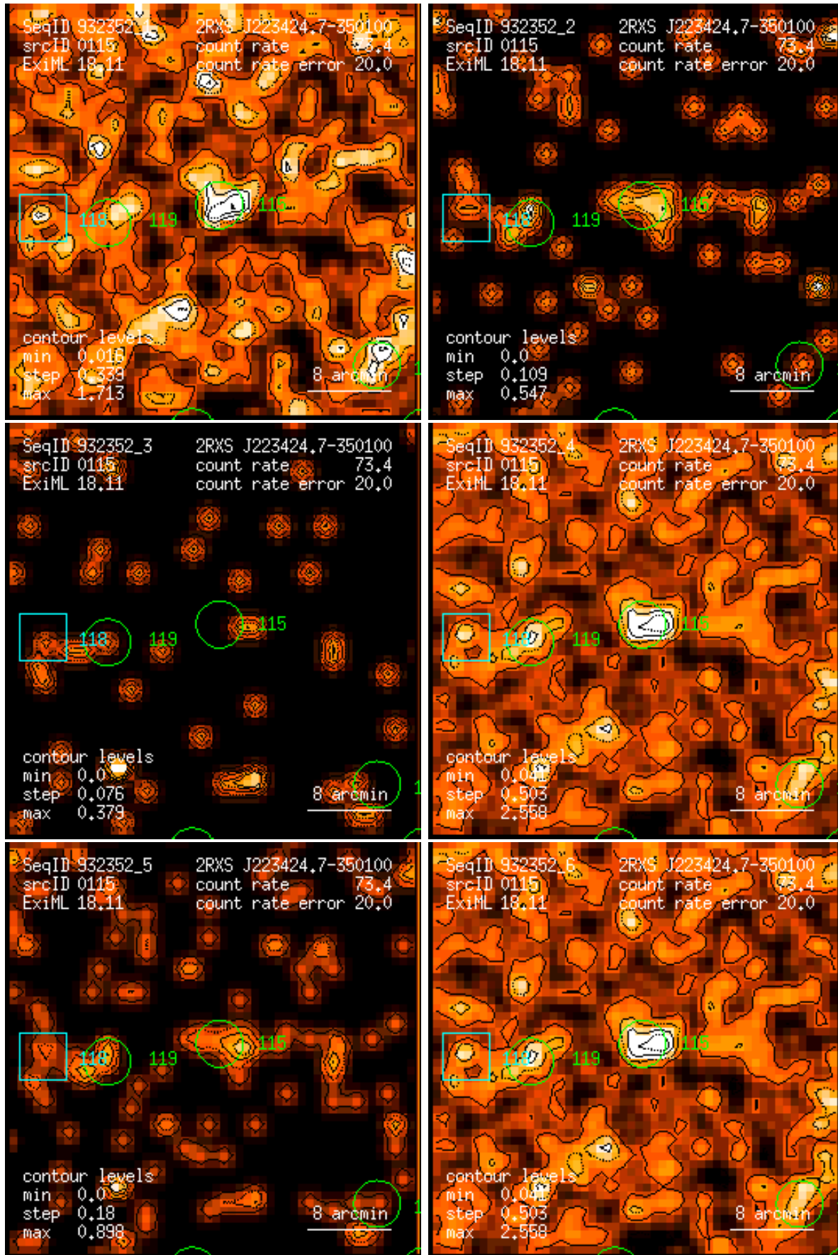
Figure 115: RASS 932352: detection 0115: band rate images, Gaussian filter: (1) PSPC channels 11 – 41, (2) 52 – 90, (3) 91 – 201, (4) 11 – 235, (5) 52 – 201, (6) 11 – 201. Broad band rates in counts/ks. Band rate contour levels in counts/ks/arcmin 2 .
