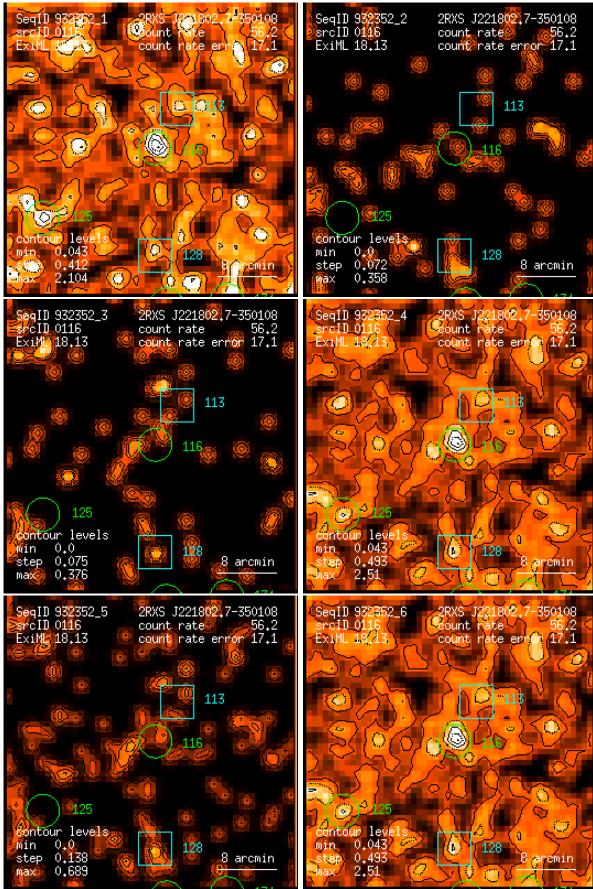
Figure 116: RASS 932352: detection 0116: band rate images, Gaussian filter: (1) PSPC channels 11 – 41, (2) 52 – 90, (3) 91 – 201, (4) 11 – 235, (5) 52 – 201, (6) 11 – 201. Broad band rates in counts/ks. Band rate contour levels in counts/ks/arcmin 2 .
