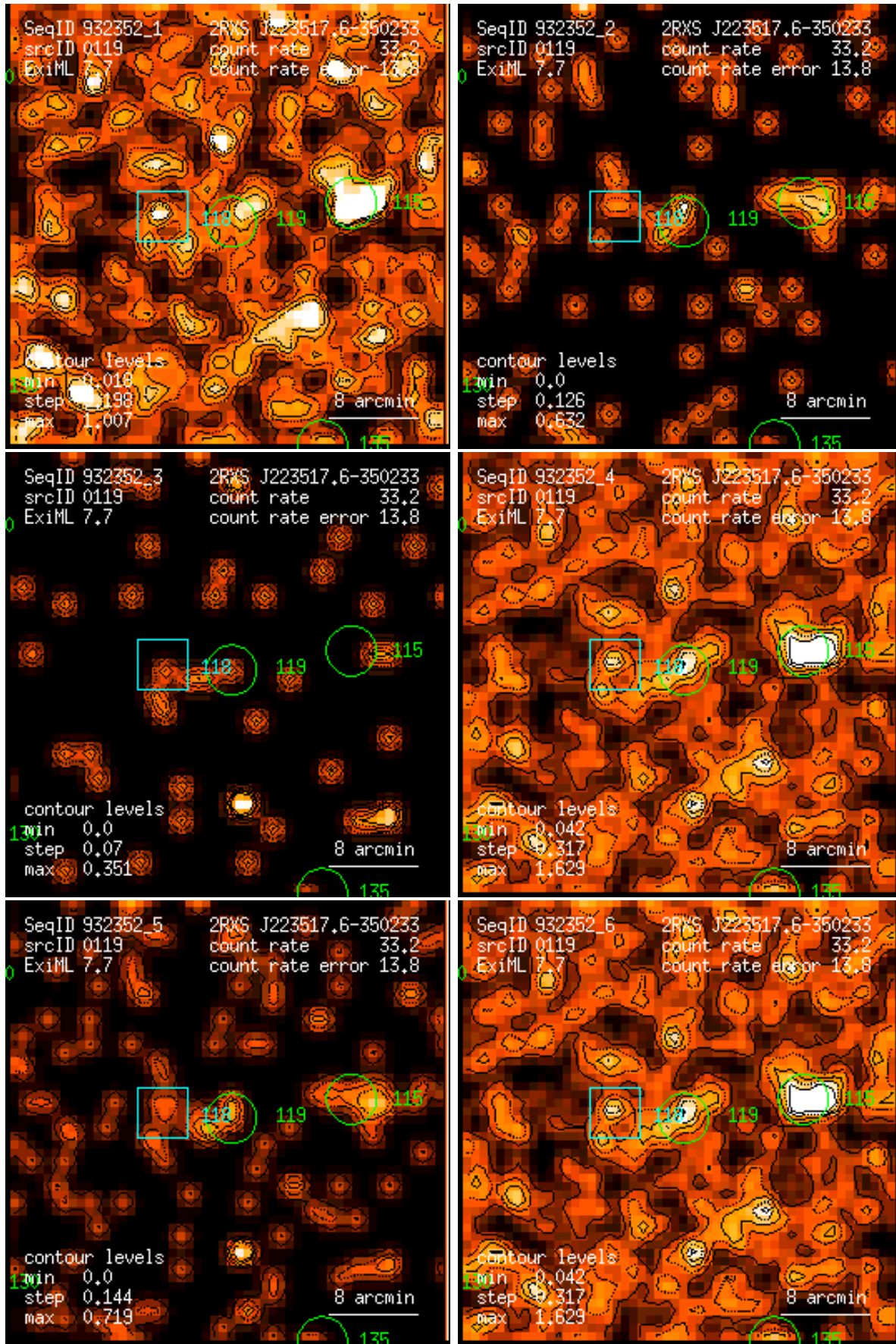
Figure 119: RASS 932352: detection 0119: band rate images, Gaussian filter: (1) PSPC channels 11 – 41, (2) 52 – 90, (3) 91 – 201, (4) 11 – 235, (5) 52 – 201, (6) 11 – 201. Broad band rates in counts/ks. Band rate contour levels in counts/ks/arcmin 2 .
