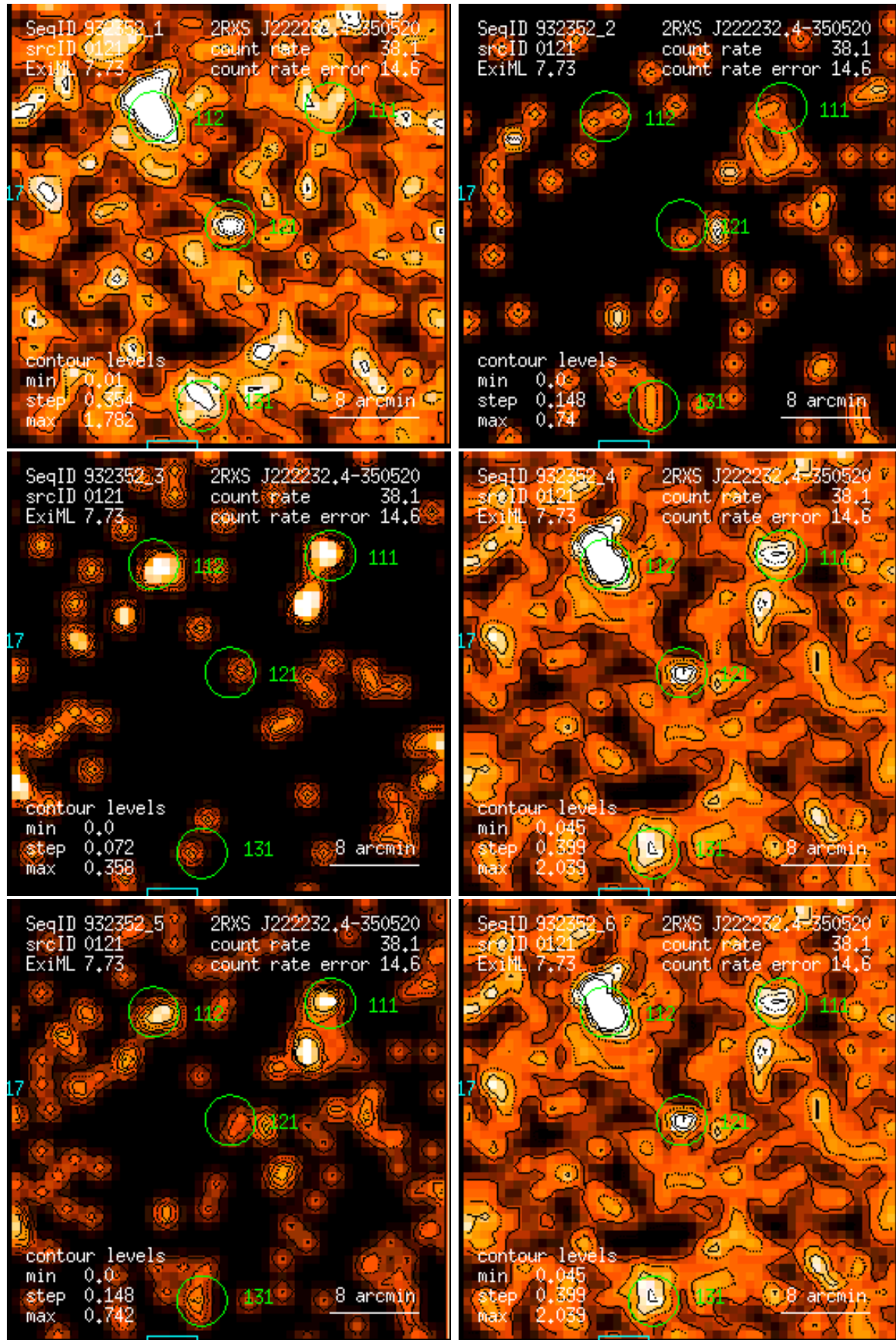
Figure 121: RASS 932352: detection 0121: band rate images, Gaussian filter: (1) PSPC channels 11 – 41, (2) 52 – 90, (3) 91 – 201, (4) 11 – 235, (5) 52 – 201, (6) 11 – 201. Broad band rates in counts/ks. Band rate contour levels in counts/ks/arcmin 2 .
