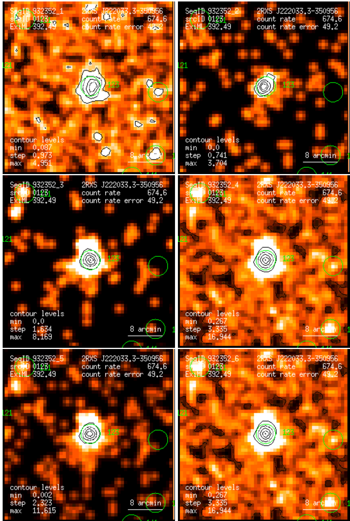
Figure 123: RASS 932352: detection 0123: band rate images, Gaussian filter: (1) PSPC channels 11 – 41, (2) 52 – 90, (3) 91 – 201, (4) 11 – 235, (5) 52 – 201, (6) 11 – 201. Broad band rates in counts/ks. Band rate contour levels in counts/ks/arcmin 2 .
