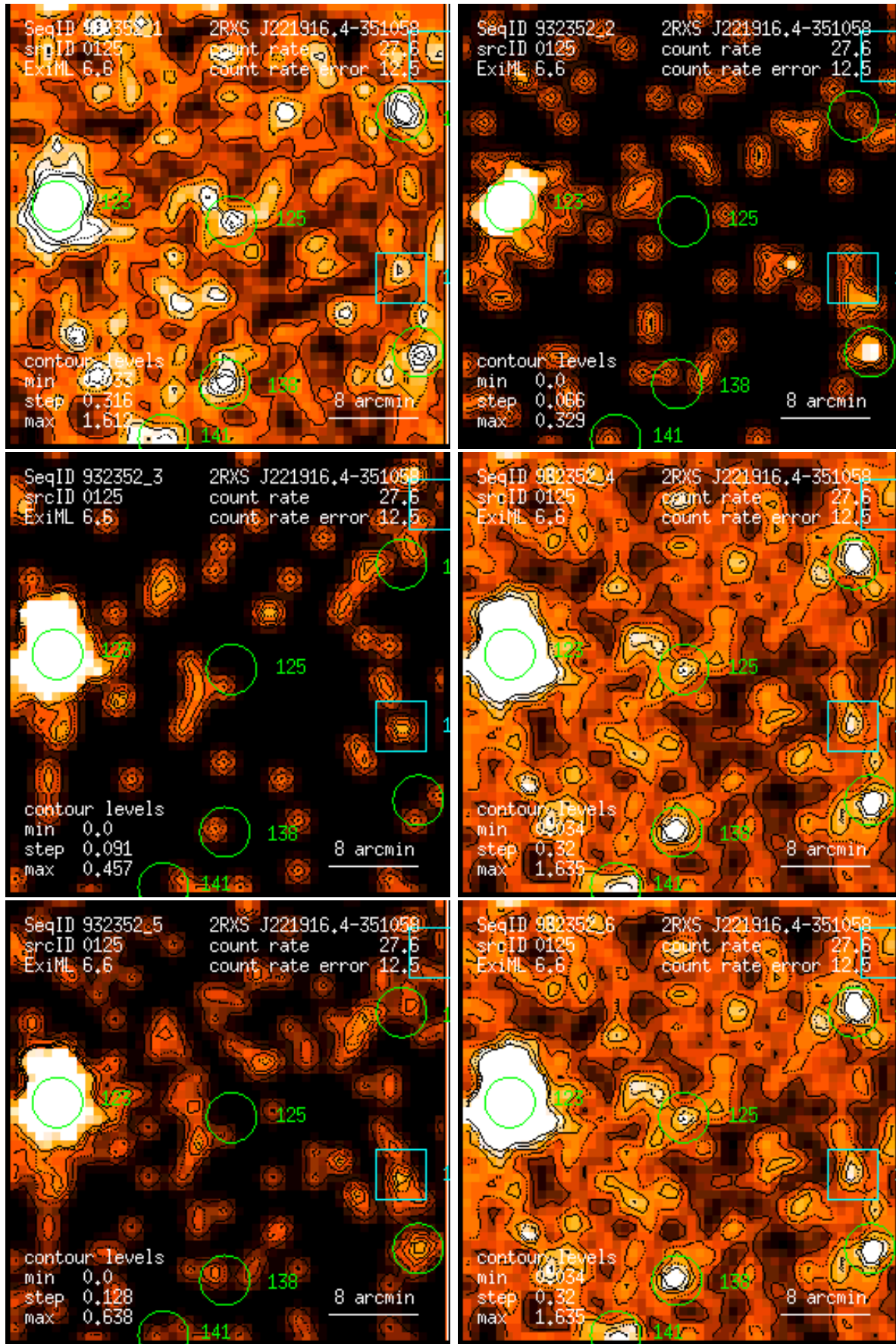
Figure 125: RASS 932352: detection 0125: band rate images, Gaussian filter: (1) PSPC channels 11 – 41, (2) 52 – 90, (3) 91 – 201, (4) 11 – 235, (5) 52 – 201, (6) 11 – 201. Broad band rates in counts/ks. Band rate contour levels in counts/ks/arcmin 2 .
