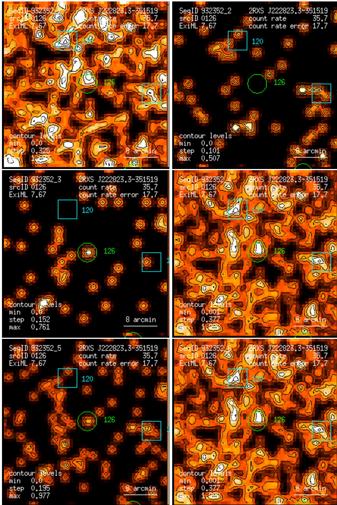
Figure 126: RASS 932352: detection 0126: band rate images, Gaussian filter: (1) PSPC channels 11 – 41, (2) 52 – 90, (3) 91 – 201, (4) 11 – 235, (5) 52 – 201, (6) 11 – 201. Broad band rates in counts/ks. Band rate contour levels in counts/ks/arcmin 2 .
