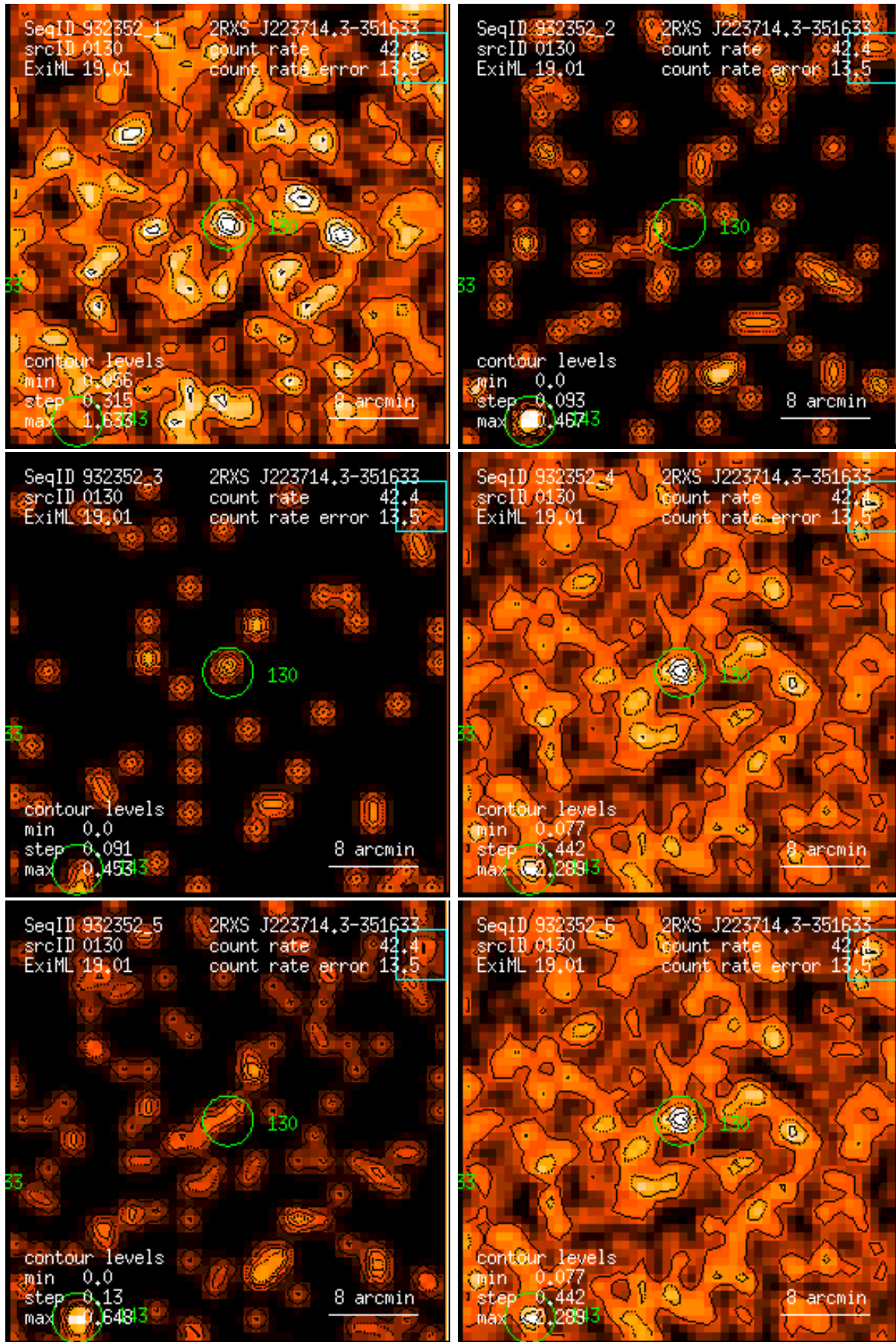
Figure 130: RASS 932352: detection 0130: band rate images, Gaussian filter: (1) PSPC channels 11 – 41, (2) 52 – 90, (3) 91 – 201, (4) 11 – 235, (5) 52 – 201, (6) 11 – 201. Broad band rates in counts/ks. Band rate contour levels in counts/ks/arcmin 2 .
