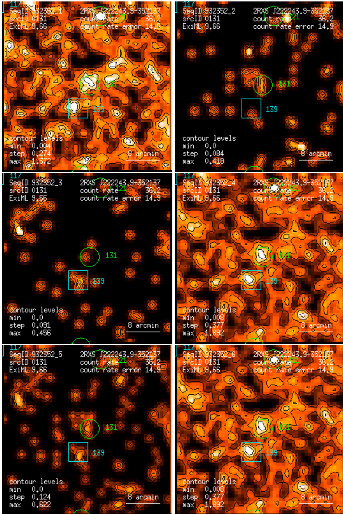
Figure 131: RASS 932352: detection 0131: band rate images, Gaussian filter: (1) PSPC channels 11 – 41, (2) 52 – 90, (3) 91 – 201, (4) 11 – 235, (5) 52 – 201, (6) 11 – 201. Broad band rates in counts/ks. Band rate contour levels in counts/ks/arcmin 2 .
