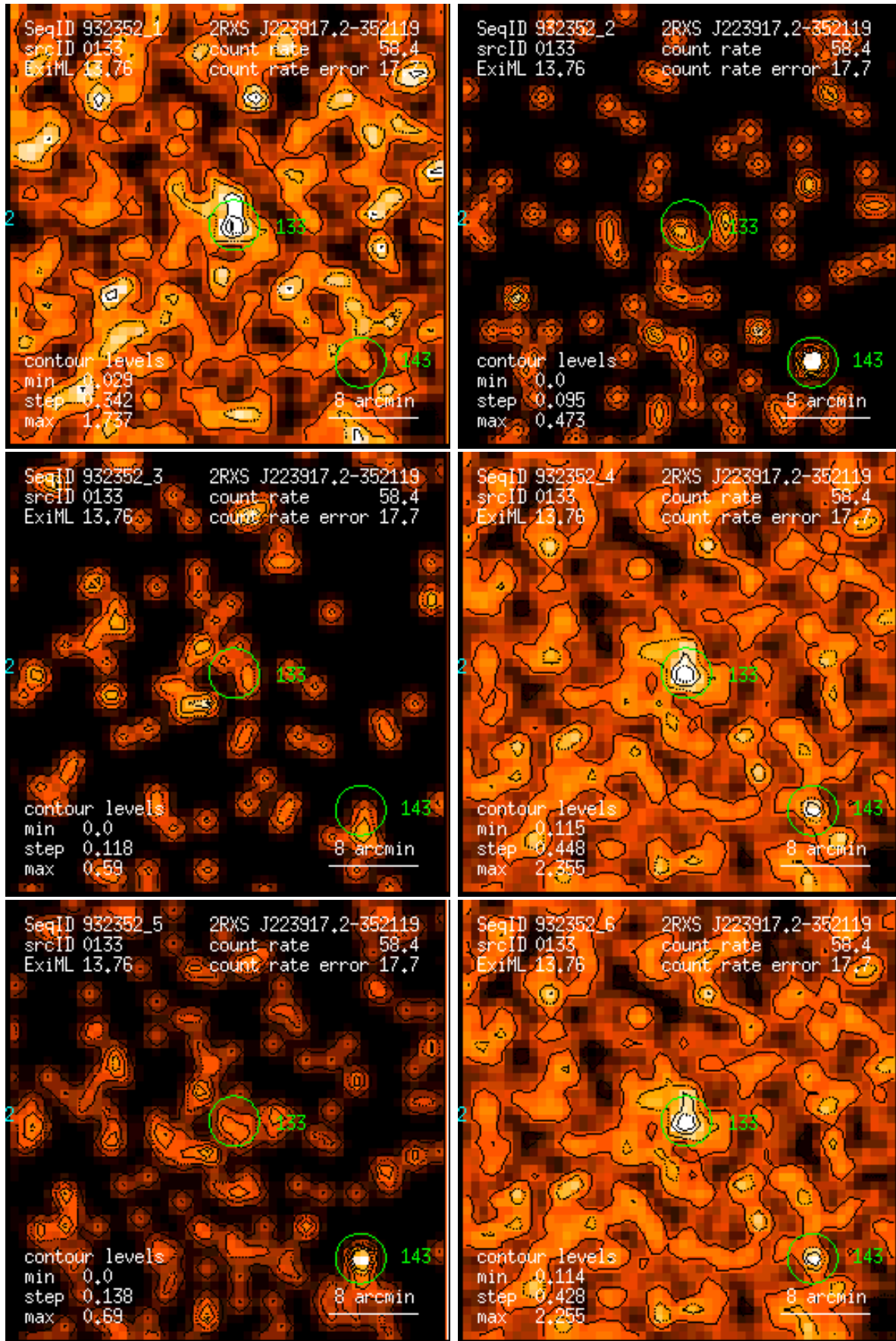
Figure 133: RASS 932352: detection 0133: band rate images, Gaussian filter: (1) PSPC channels 11 – 41, (2) 52 – 90, (3) 91 – 201, (4) 11 – 235, (5) 52 – 201, (6) 11 – 201. Broad band rates in counts/ks. Band rate contour levels in counts/ks/arcmin 2 .
