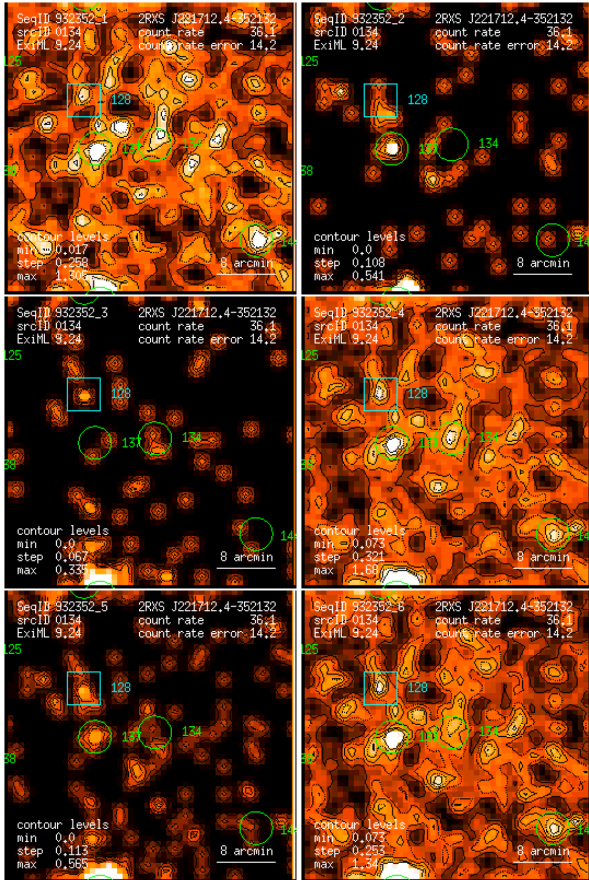
Figure 134: RASS 932352: detection 0134: band rate images, Gaussian filter: (1) PSPC channels 11 – 41, (2) 52 – 90, (3) 91 – 201, (4) 11 – 235, (5) 52 – 201, (6) 11 – 201. Broad band rates in counts/ks. Band rate contour levels in counts/ks/arcmin 2 .
