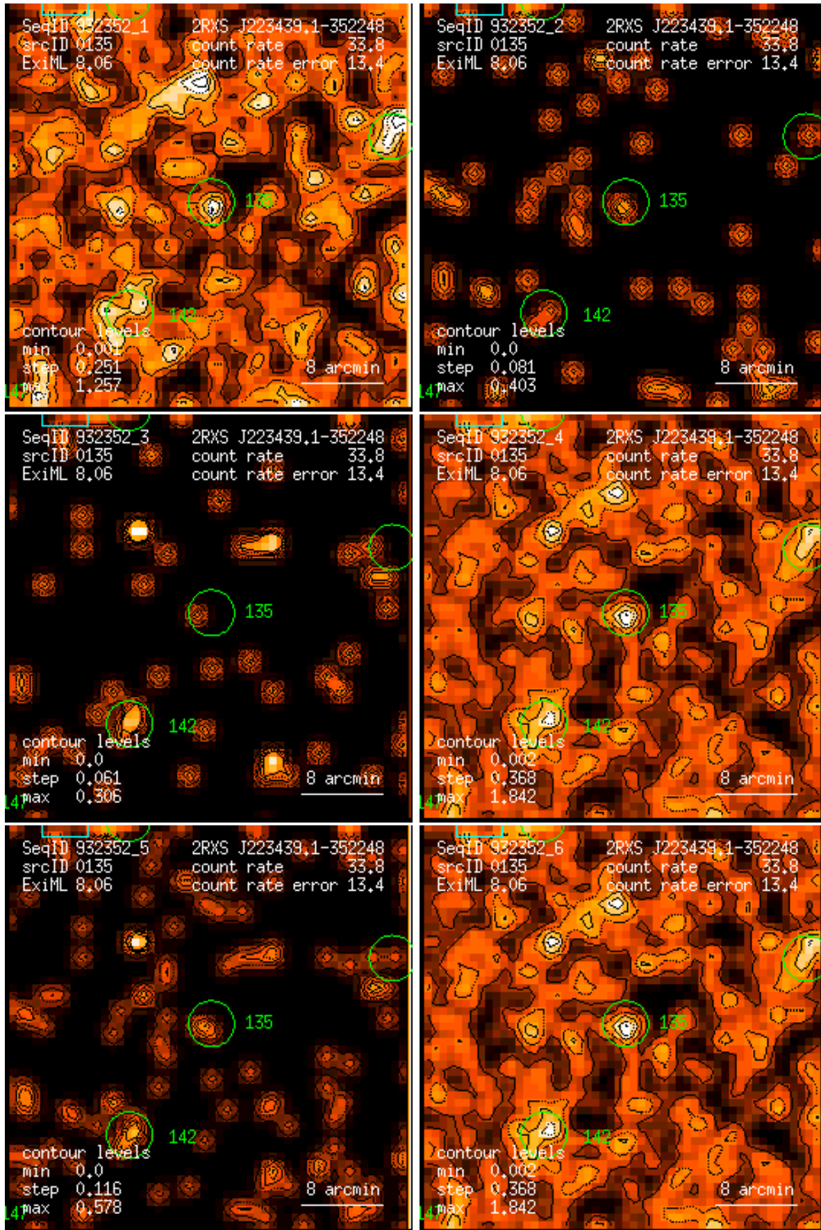
Figure 135: RASS 932352: detection 0135: band rate images, Gaussian filter: (1) PSPC channels 11 – 41, (2) 52 – 90, (3) 91 – 201, (4) 11 – 235, (5) 52 – 201, (6) 11 – 201. Broad band rates in counts/ks. Band rate contour levels in counts/ks/arcmin 2 .
