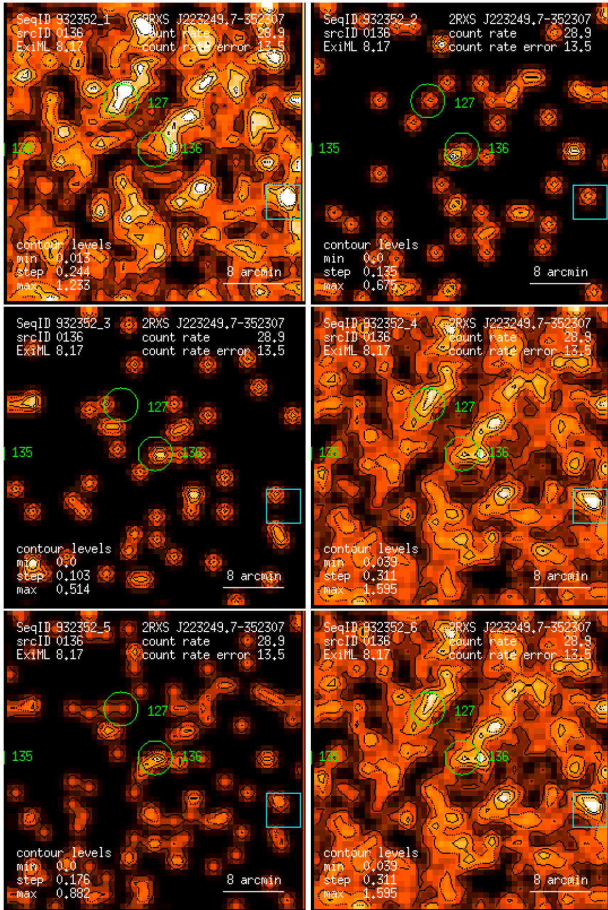
Figure 136: RASS 932352: detection 0136: band rate images, Gaussian filter: (1) PSPC channels 11 – 41, (2) 52 – 90, (3) 91 – 201, (4) 11 – 235, (5) 52 – 201, (6) 11 – 201. Broad band rates in counts/ks. Band rate contour levels in counts/ks/arcmin 2 .
