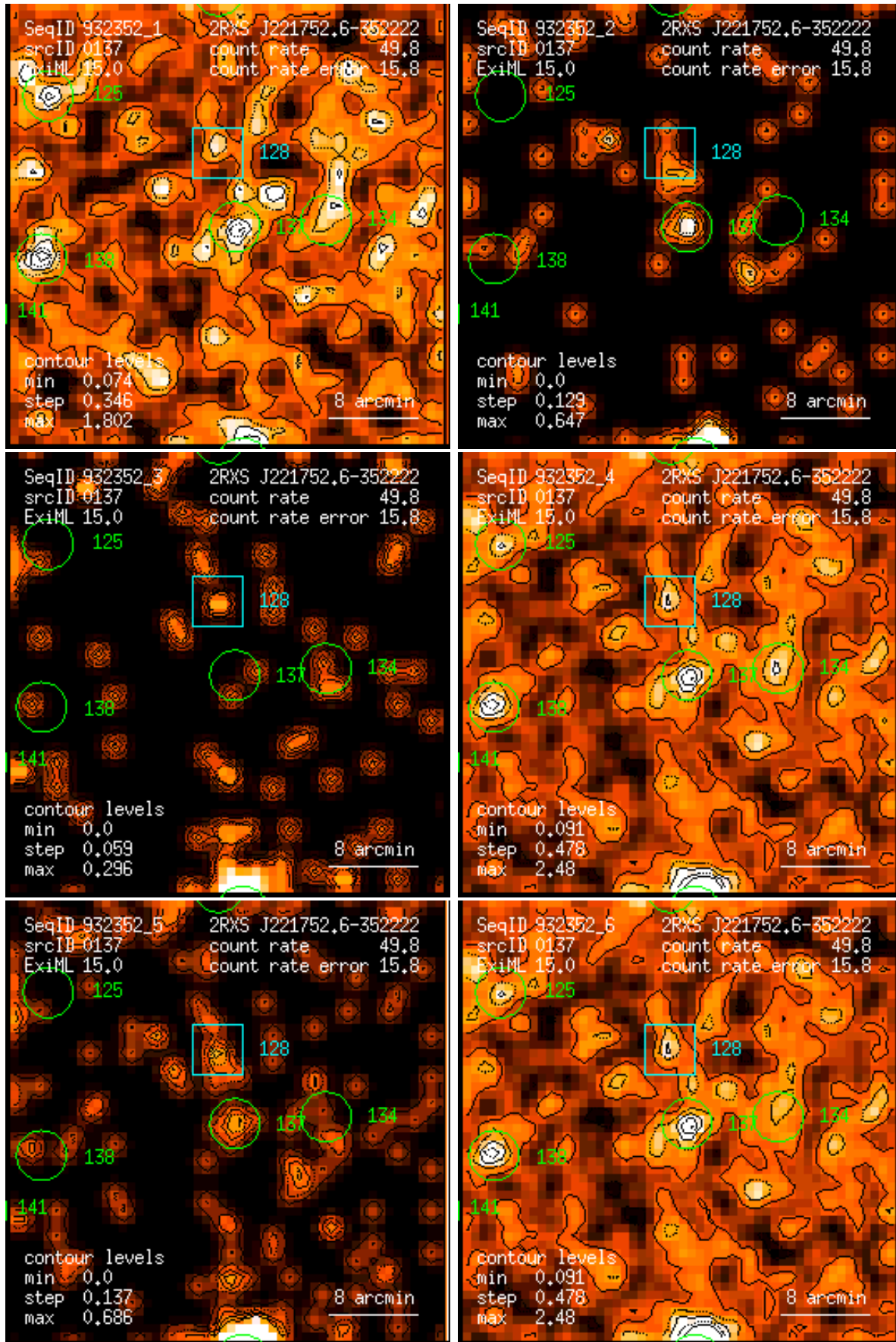
Figure 137: RASS 932352: detection 0137: band rate images, Gaussian filter: (1) PSPC channels 11 – 41, (2) 52 – 90, (3) 91 – 201, (4) 11 – 235, (5) 52 – 201, (6) 11 – 201. Broad band rates in counts/ks. Band rate contour levels in counts/ks/arcmin 2 .
