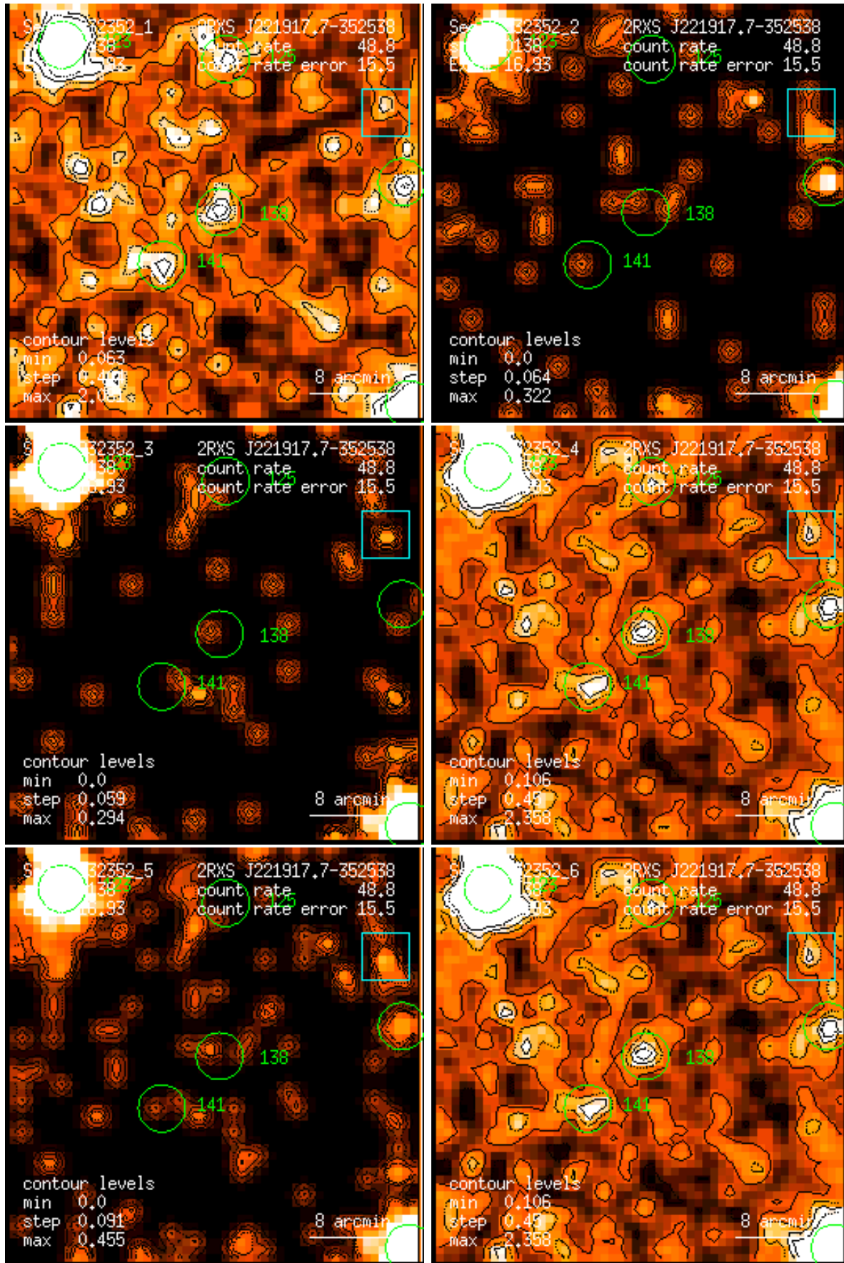
Figure 138: RASS 932352: detection 0138: band rate images, Gaussian filter: (1) PSPC channels 11 – 41, (2) 52 – 90, (3) 91 – 201, (4) 11 – 235, (5) 52 – 201, (6) 11 – 201. Broad band rates in counts/ks. Band rate contour levels in counts/ks/arcmin 2 .
