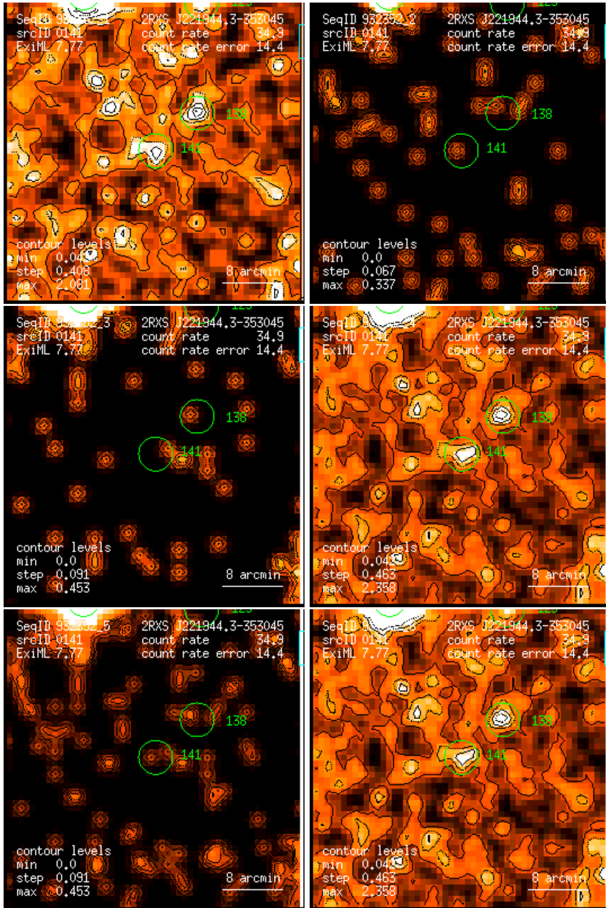
Figure 141: RASS 932352: detection 0141: band rate images, Gaussian filter: (1) PSPC channels 11 – 41, (2) 52 – 90, (3) 91 – 201, (4) 11 – 235, (5) 52 – 201, (6) 11 – 201. Broad band rates in counts/ks. Band rate contour levels in counts/ks/arcmin 2 .
