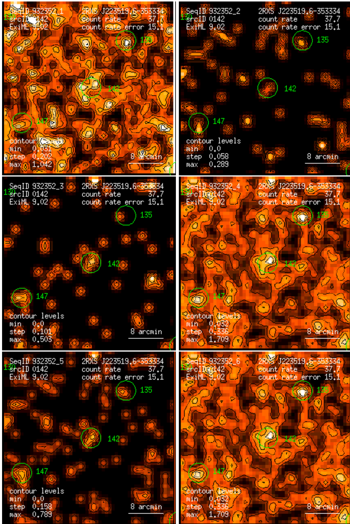
Figure 142: RASS 932352: detection 0142: band rate images, Gaussian filter: (1) PSPC channels 11 – 41, (2) 52 – 90, (3) 91 – 201, (4) 11 – 235, (5) 52 – 201, (6) 11 – 201. Broad band rates in counts/ks. Band rate contour levels in counts/ks/arcmin 2 .
