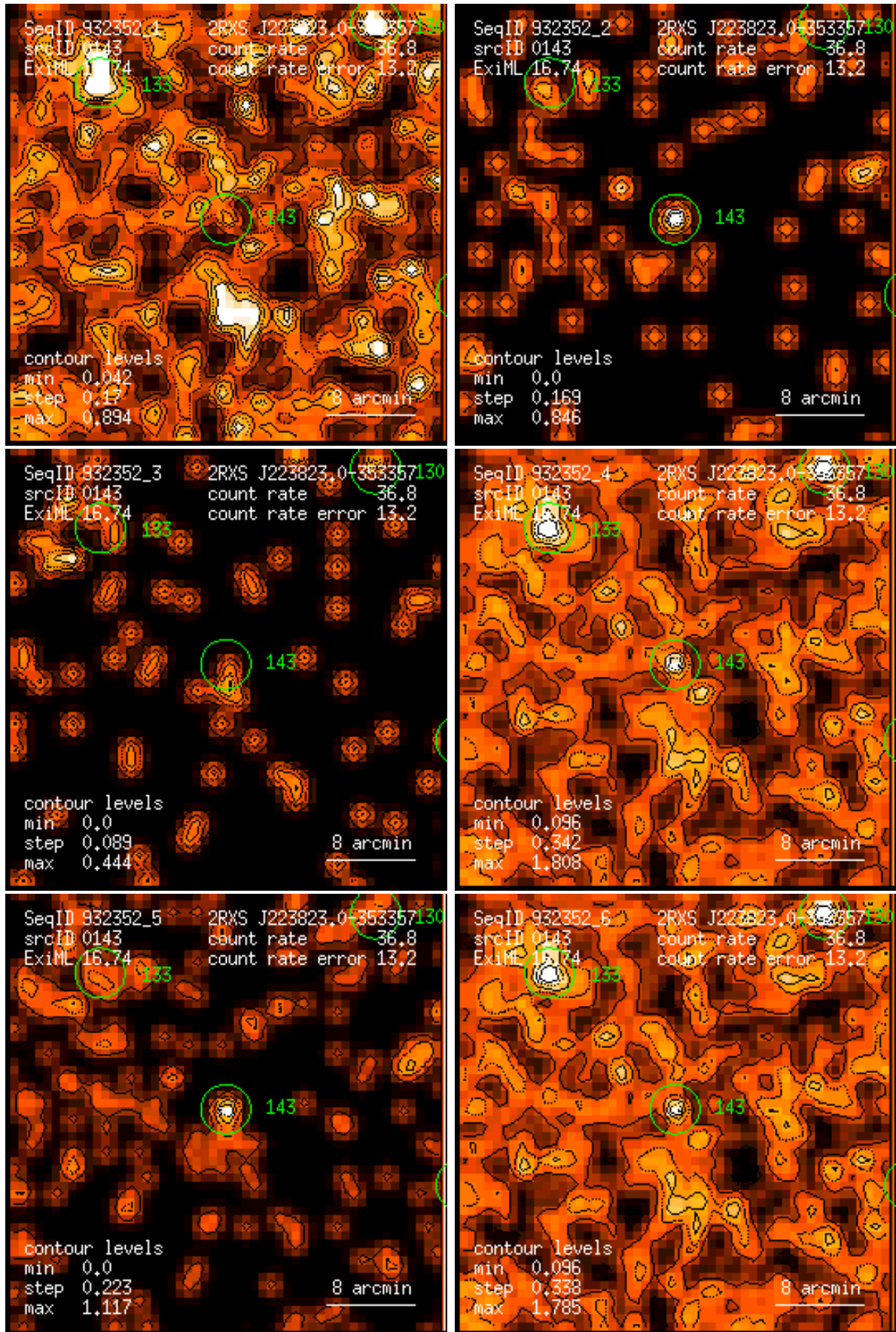
Figure 143: RASS 932352: detection 0143: band rate images, Gaussian filter: (1) PSPC channels 11 – 41, (2) 52 – 90, (3) 91 – 201, (4) 11 – 235, (5) 52 – 201, (6) 11 – 201. Broad band rates in counts/ks. Band rate contour levels in counts/ks/arcmin 2 .
