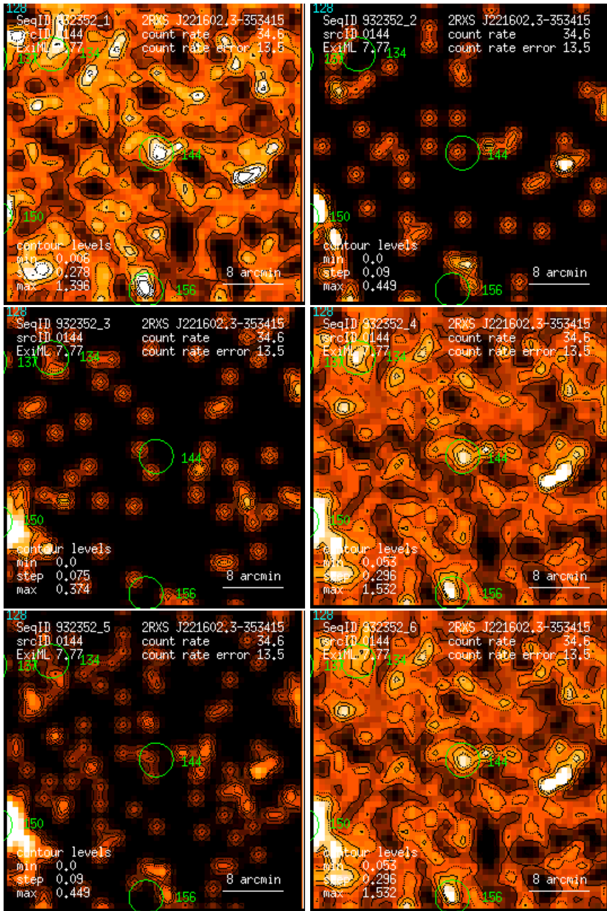
Figure 144: RASS 932352: detection 0144: band rate images, Gaussian filter: (1) PSPC channels 11 – 41, (2) 52 – 90, (3) 91 – 201, (4) 11 – 235, (5) 52 – 201, (6) 11 – 201. Broad band rates in counts/ks. Band rate contour levels in counts/ks/arcmin 2 .
