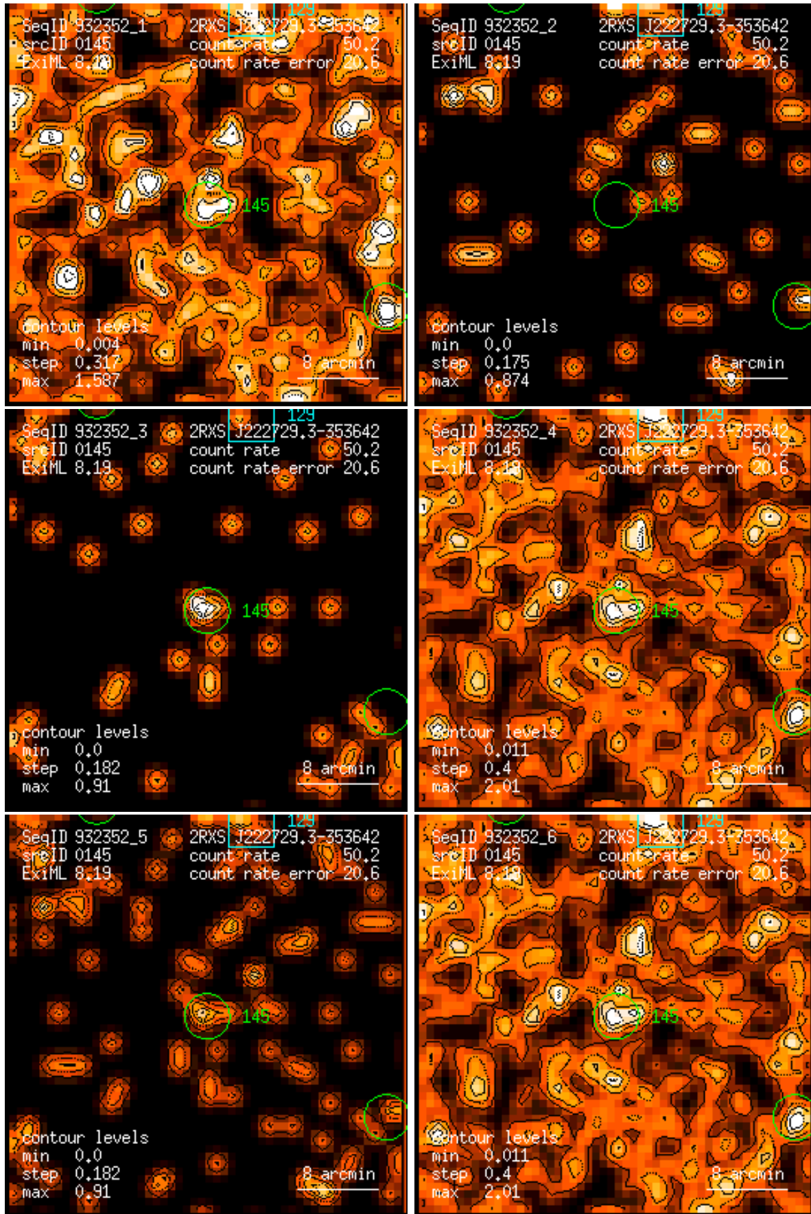
Figure 145: RASS 932352: detection 0145: band rate images, Gaussian filter: (1) PSPC channels 11 – 41, (2) 52 – 90, (3) 91 – 201, (4) 11 – 235, (5) 52 – 201, (6) 11 – 201. Broad band rates in counts/ks. Band rate contour levels in counts/ks/arcmin 2 .
