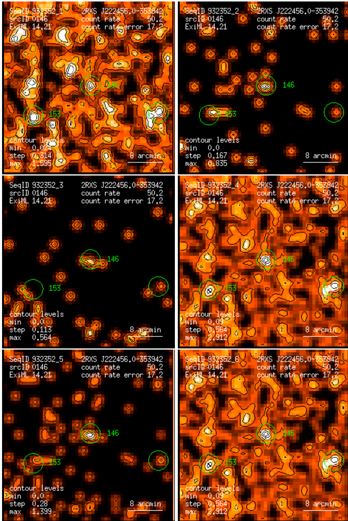
Figure 146: RASS 932352: detection 0146: band rate images, Gaussian filter: (1) PSPC channels 11 – 41, (2) 52 – 90, (3) 91 – 201, (4) 11 – 235, (5) 52 – 201, (6) 11 – 201. Broad band rates in counts/ks. Band rate contour levels in counts/ks/arcmin 2 .
