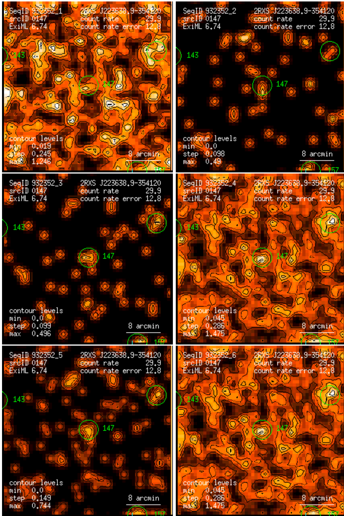
Figure 147: RASS 932352: detection 0147: band rate images, Gaussian filter: (1) PSPC channels 11 – 41, (2) 52 – 90, (3) 91 – 201, (4) 11 – 235, (5) 52 – 201, (6) 11 – 201. Broad band rates in counts/ks. Band rate contour levels in counts/ks/arcmin 2 .
