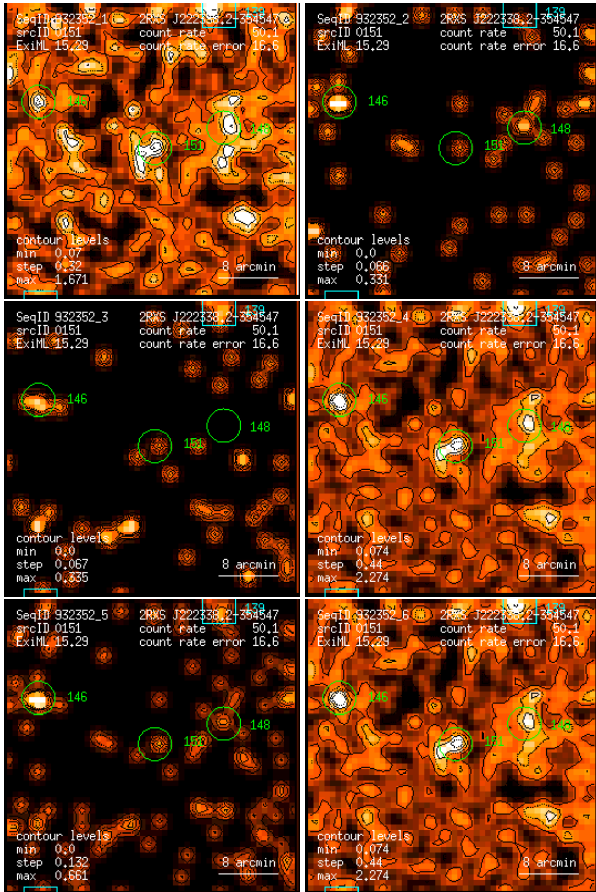
Figure 151: RASS 932352: detection 0151: band rate images, Gaussian filter: (1) PSPC channels 11 – 41, (2) 52 – 90, (3) 91 – 201, (4) 11 – 235, (5) 52 – 201, (6) 11 – 201. Broad band rates in counts/ks. Band rate contour levels in counts/ks/arcmin 2 .
