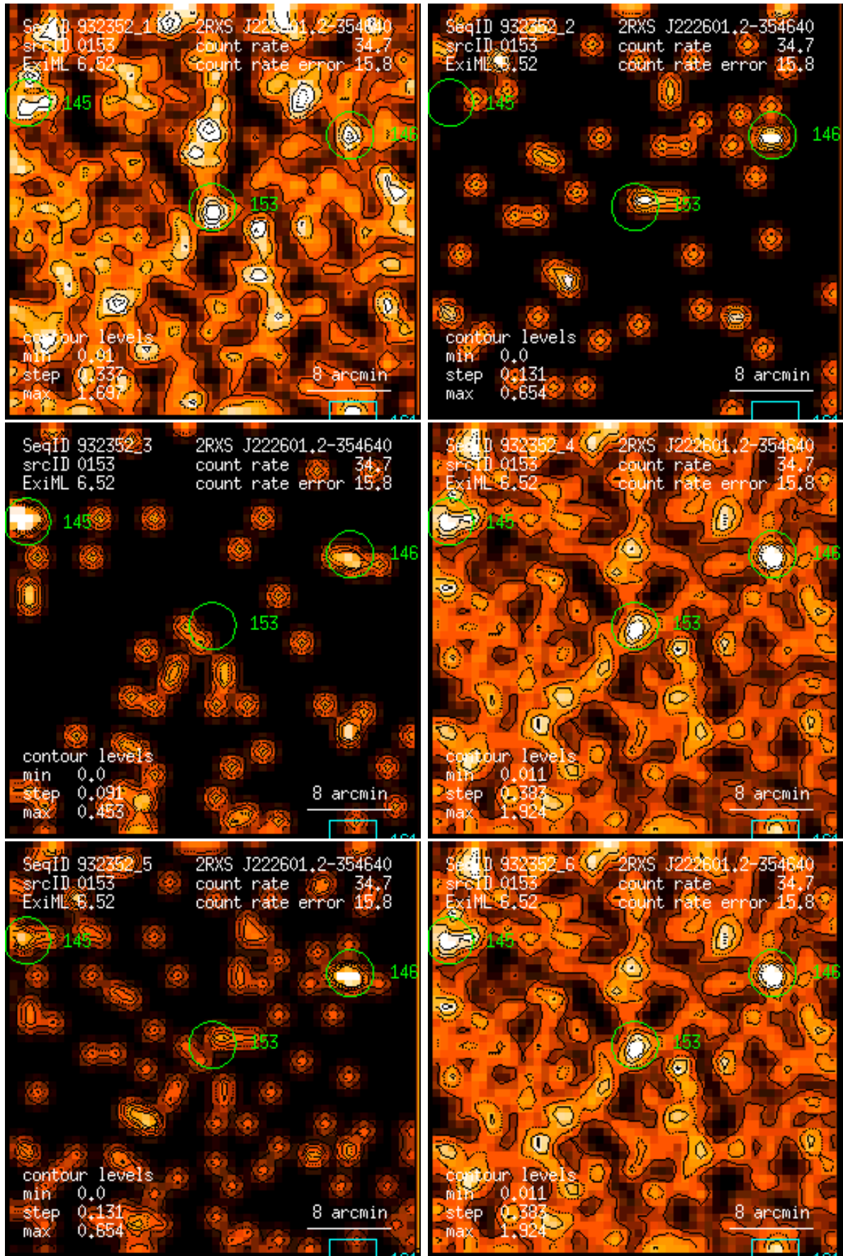
Figure 153: RASS 932352: detection 0153: band rate images, Gaussian filter: (1) PSPC channels 11 – 41, (2) 52 – 90, (3) 91 – 201, (4) 11 – 235, (5) 52 – 201, (6) 11 – 201. Broad band rates in counts/ks. Band rate contour levels in counts/ks/arcmin 2 .
