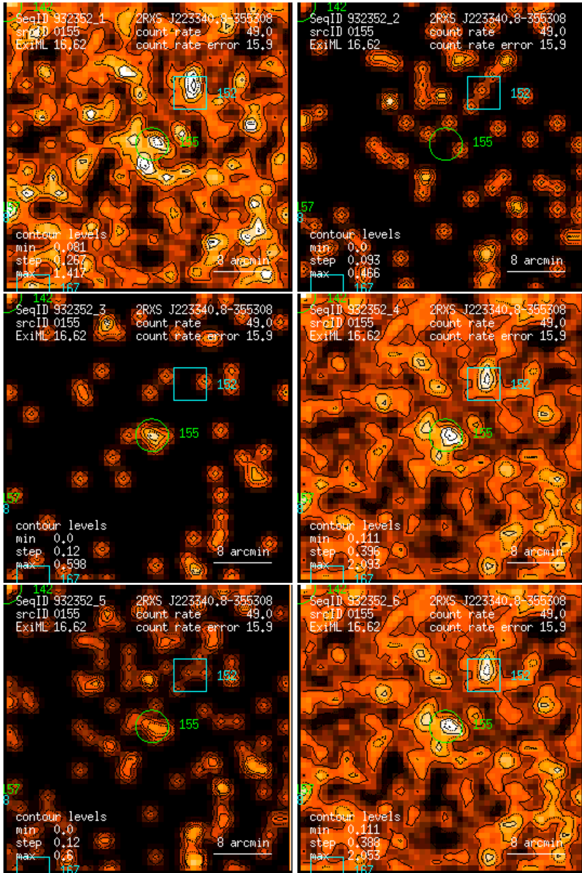
Figure 155: RASS 932352: detection 0155: band rate images, Gaussian filter: (1) PSPC channels 11 – 41, (2) 52 – 90, (3) 91 – 201, (4) 11 – 235, (5) 52 – 201, (6) 11 – 201. Broad band rates in counts/ks. Band rate contour levels in counts/ks/arcmin 2 .
