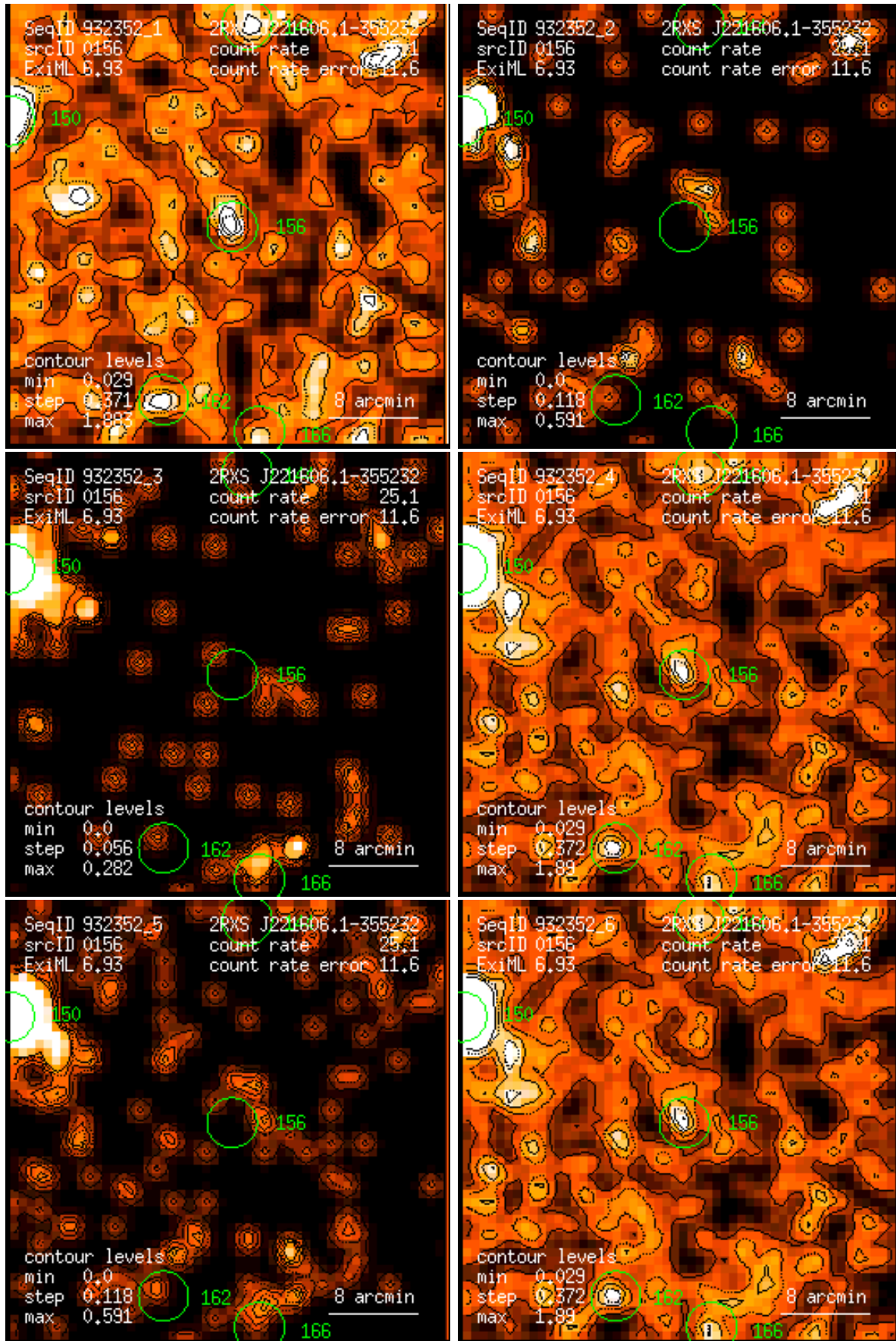
Figure 156: RASS 932352: detection 0156: band rate images, Gaussian filter: (1) PSPC channels 11 – 41, (2) 52 – 90, (3) 91 – 201, (4) 11 – 235, (5) 52 – 201, (6) 11 – 201. Broad band rates in counts/ks. Band rate contour levels in counts/ks/arcmin 2 .
