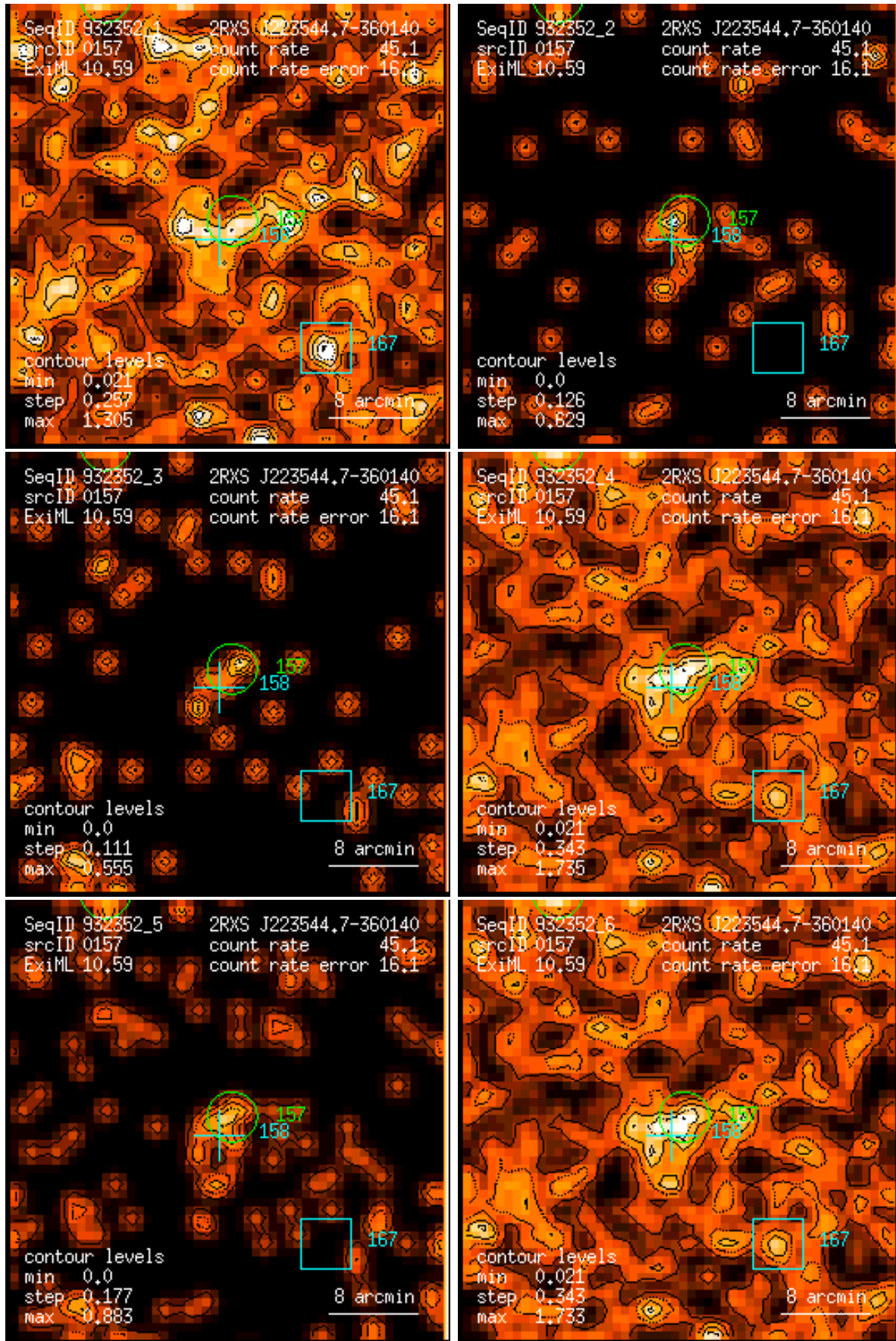
Figure 157: RASS 932352: detection 0157: band rate images, Gaussian filter: (1) PSPC channels 11 – 41, (2) 52 – 90, (3) 91 – 201, (4) 11 – 235, (5) 52 – 201, (6) 11 – 201. Broad band rates in counts/ks. Band rate contour levels in counts/ks/arcmin 2 .
