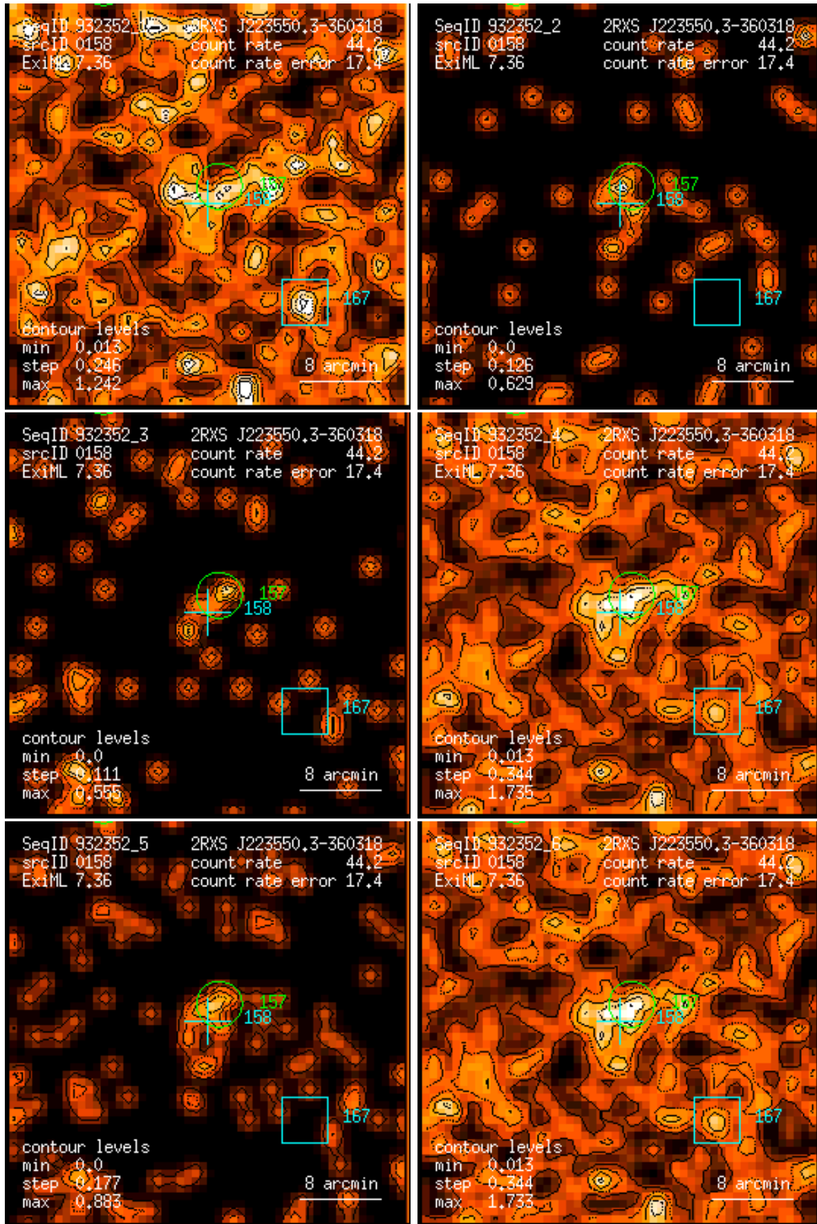
Figure 158: RASS 932352: detection 0158: band rate images, Gaussian filter: (1) PSPC channels 11 – 41, (2) 52 – 90, (3) 91 – 201, (4) 11 – 235, (5) 52 – 201, (6) 11 – 201. Broad band rates in counts/ks. Band rate contour levels in counts/ks/arcmin 2 .
