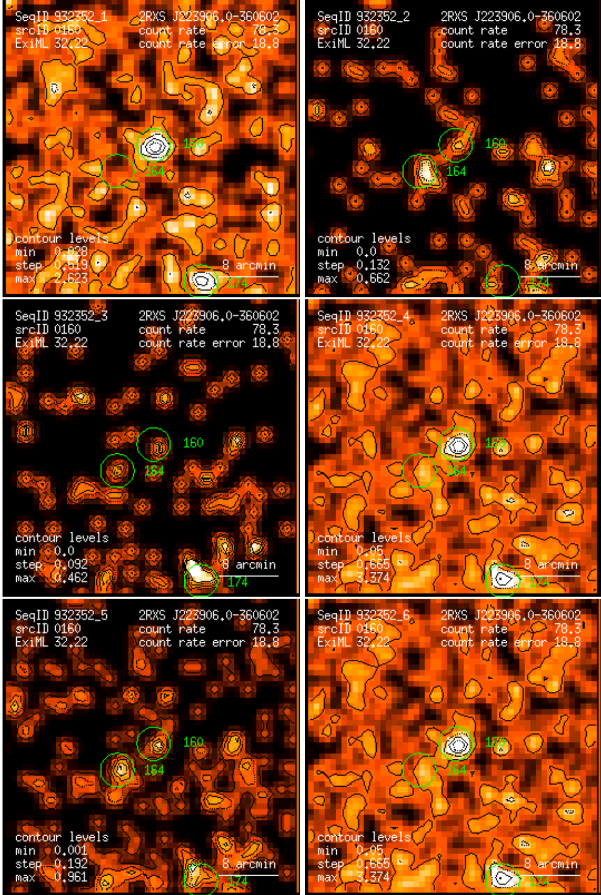
Figure 160: RASS 932352: detection 0160: band rate images, Gaussian filter: (1) PSPC channels 11 – 41, (2) 52 – 90, (3) 91 – 201, (4) 11 – 235, (5) 52 – 201, (6) 11 – 201. Broad band rates in counts/ks. Band rate contour levels in counts/ks/arcmin 2 .
