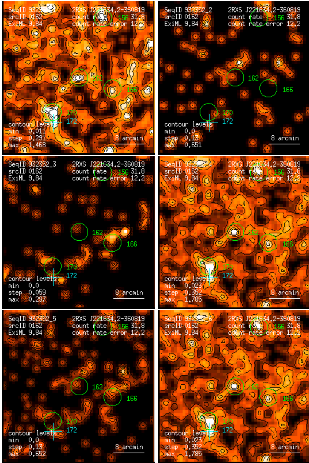
Figure 162: RASS 932352: detection 0162: band rate images, Gaussian filter: (1) PSPC channels 11 – 41, (2) 52 – 90, (3) 91 – 201, (4) 11 – 235, (5) 52 – 201, (6) 11 – 201. Broad band rates in counts/ks. Band rate contour levels in counts/ks/arcmin 2 .
