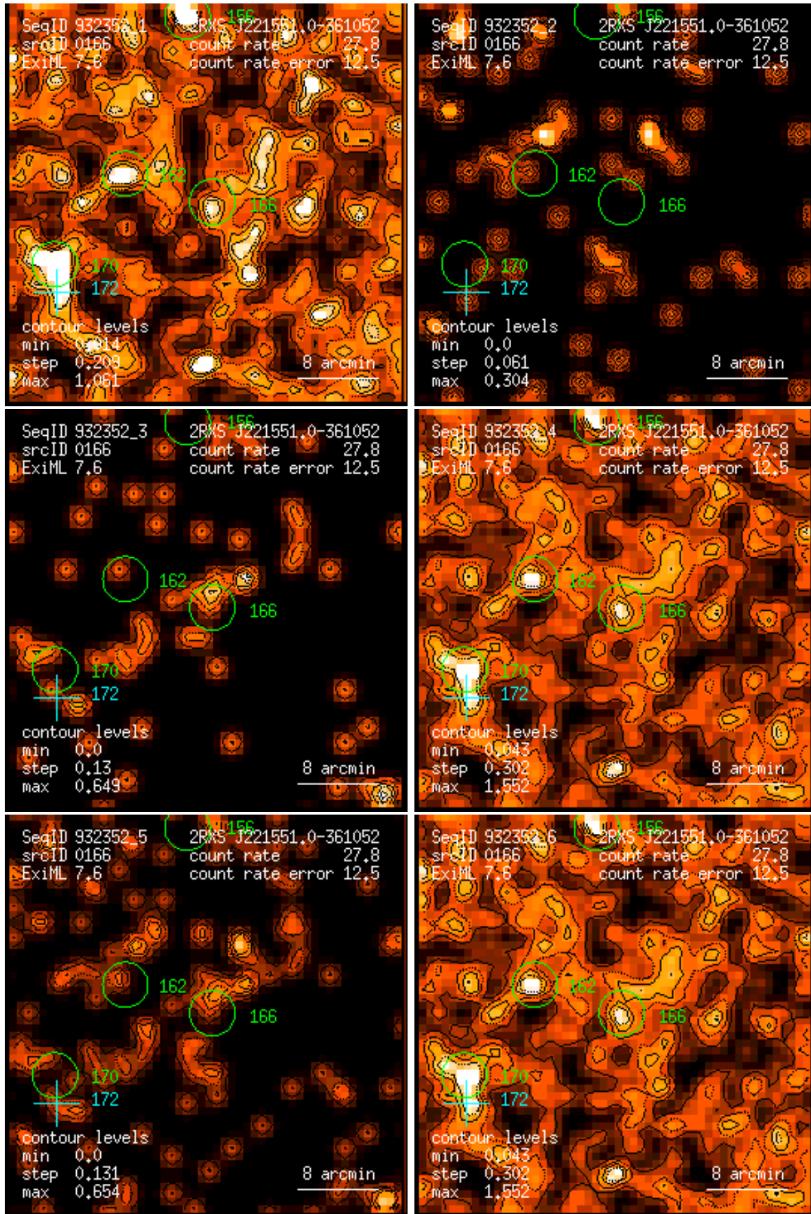
Figure 166: RASS 932352: detection 0166: band rate images, Gaussian filter: (1) PSPC channels 11 – 41, (2) 52 – 90, (3) 91 – 201, (4) 11 – 235, (5) 52 – 201, (6) 11 – 201. Broad band rates in counts/ks. Band rate contour levels in counts/ks/arcmin 2 .
