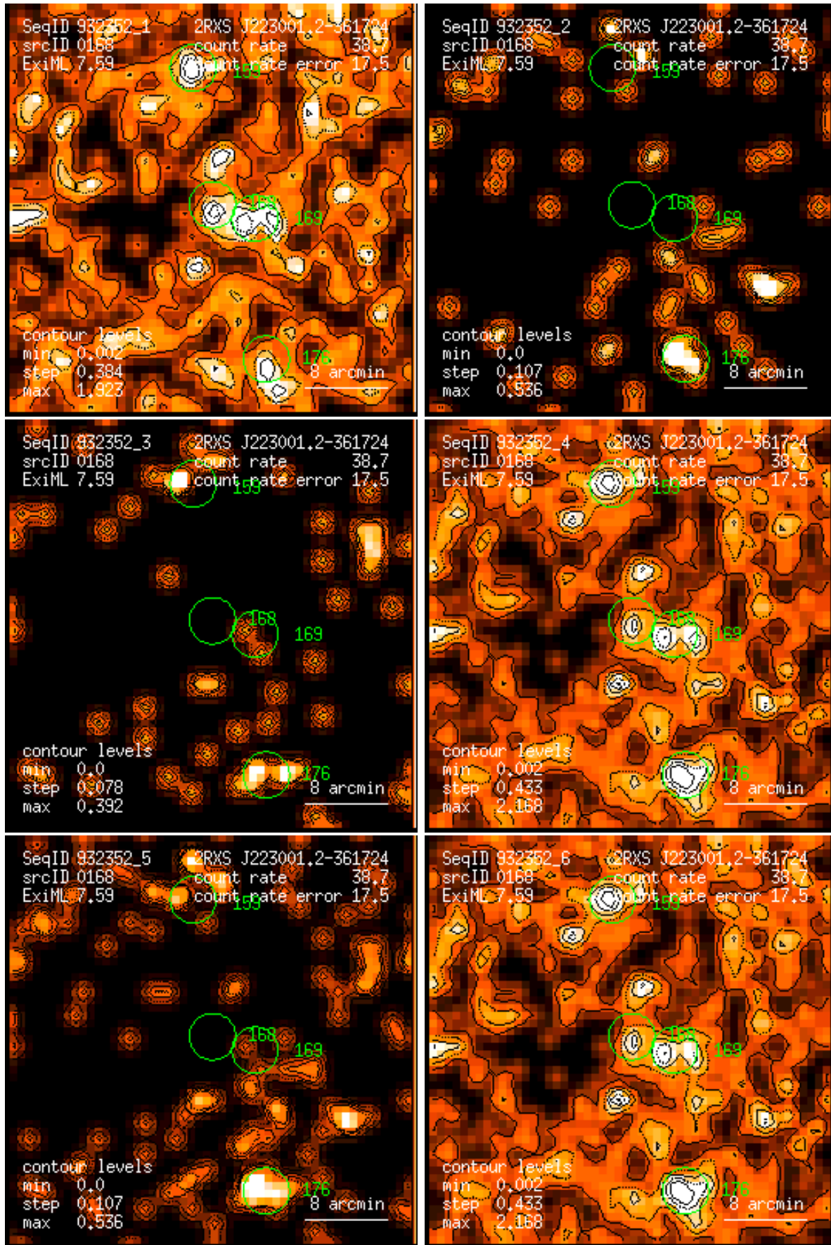
Figure 168: RASS 932352: detection 0168: band rate images, Gaussian filter: (1) PSPC channels 11 – 41, (2) 52 – 90, (3) 91 – 201, (4) 11 – 235, (5) 52 – 201, (6) 11 – 201. Broad band rates in counts/ks. Band rate contour levels in counts/ks/arcmin 2 .
