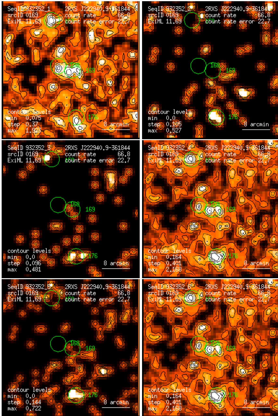
Figure 169: RASS 932352: detection 0169: band rate images, Gaussian filter: (1) PSPC channels 11 – 41, (2) 52 – 90, (3) 91 – 201, (4) 11 – 235, (5) 52 – 201, (6) 11 – 201. Broad band rates in counts/ks. Band rate contour levels in counts/ks/arcmin 2 .
