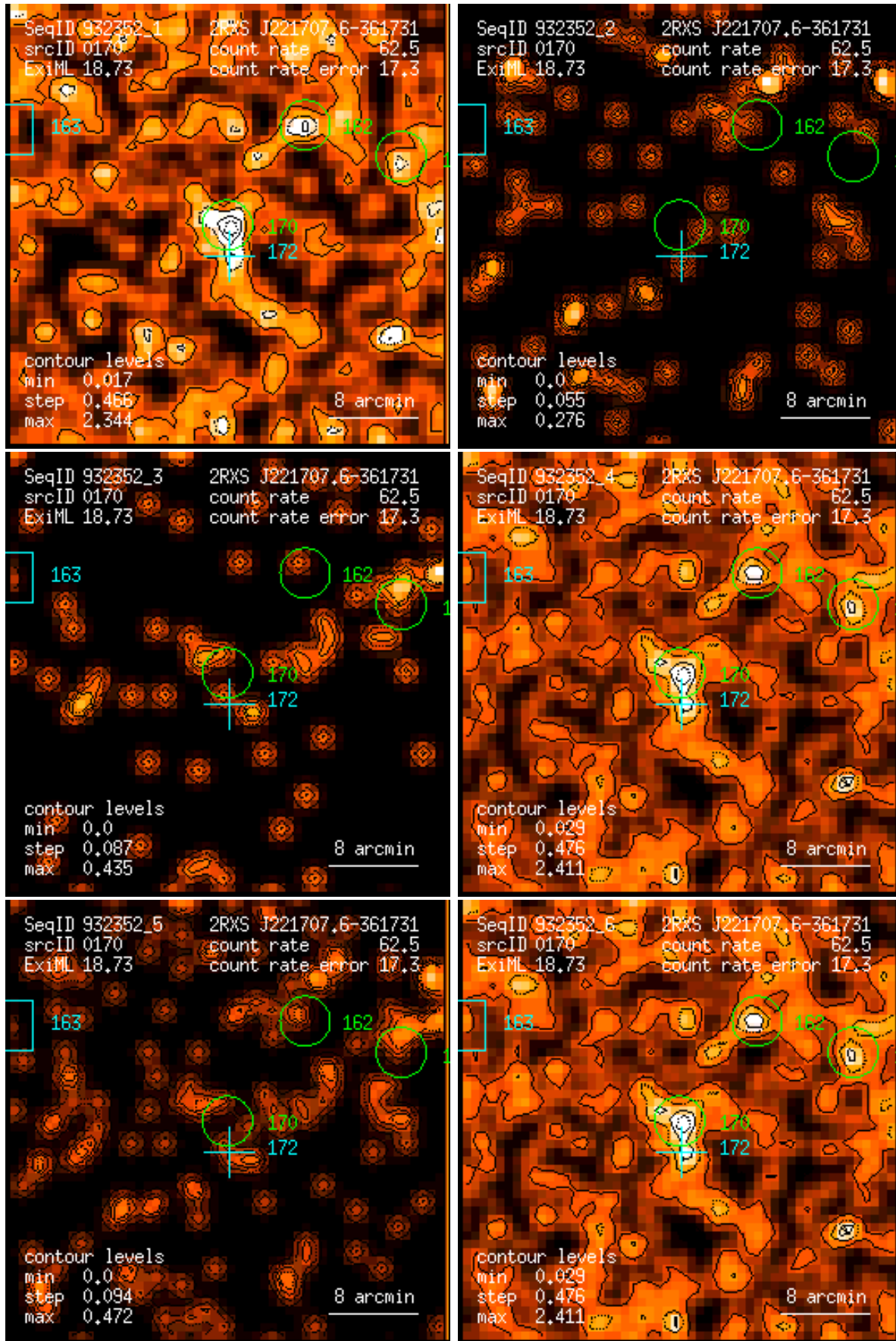
Figure 170: RASS 932352: detection 0170: band rate images, Gaussian filter: (1) PSPC channels 11 – 41, (2) 52 – 90, (3) 91 – 201, (4) 11 – 235, (5) 52 – 201, (6) 11 – 201. Broad band rates in counts/ks. Band rate contour levels in counts/ks/arcmin 2 .
