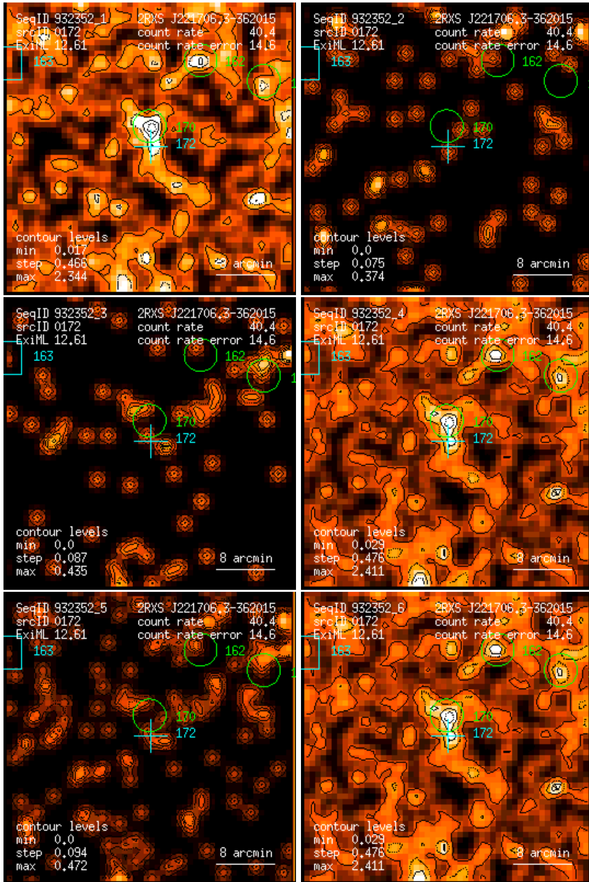
Figure 172: RASS 932352: detection 0172: band rate images, Gaussian filter: (1) PSPC channels 11 – 41, (2) 52 – 90, (3) 91 – 201, (4) 11 – 235, (5) 52 – 201, (6) 11 – 201. Broad band rates in counts/ks. Band rate contour levels in counts/ks/arcmin 2 .
