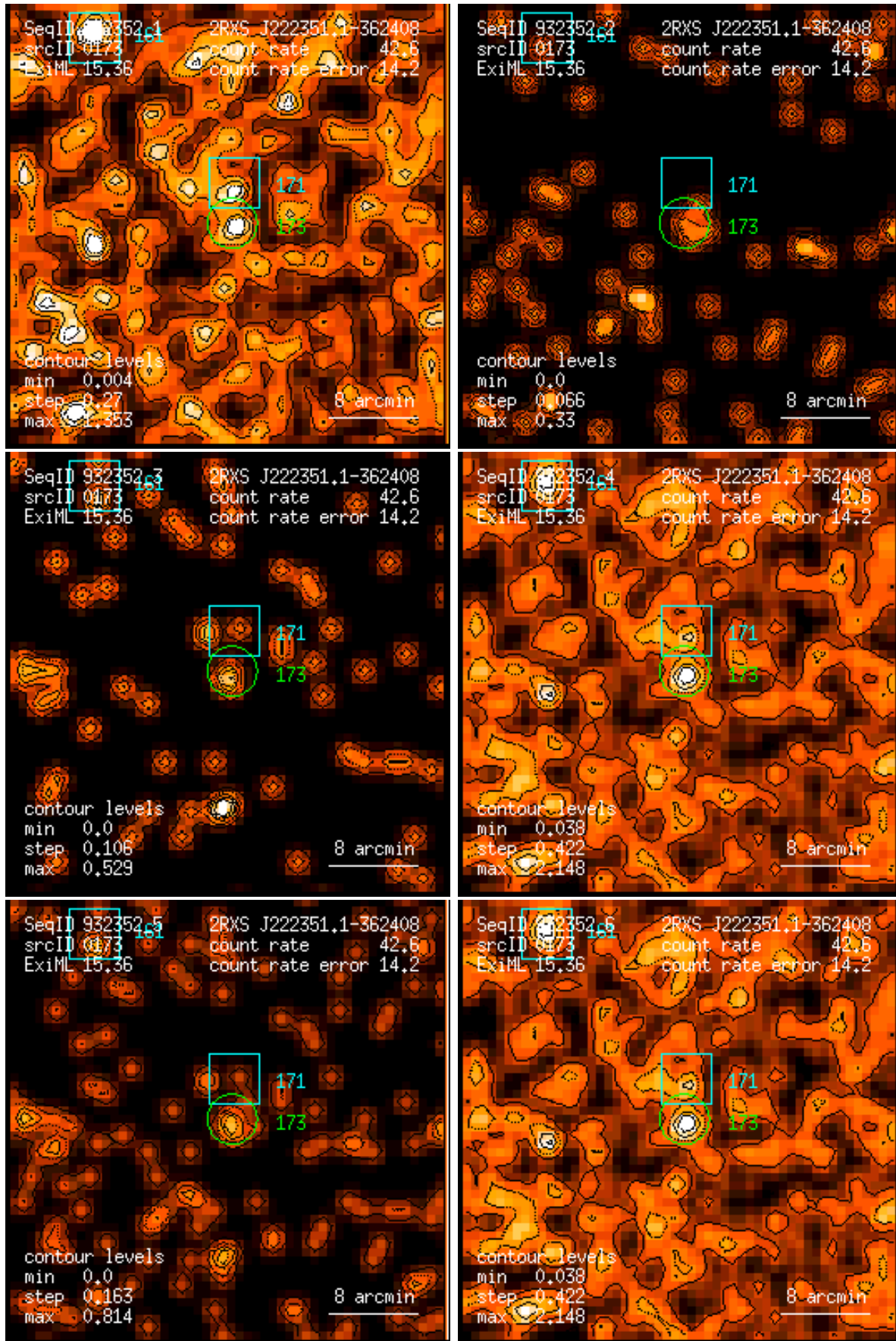
Figure 173: RASS 932352: detection 0173: band rate images, Gaussian filter: (1) PSPC channels 11 – 41, (2) 52 – 90, (3) 91 – 201, (4) 11 – 235, (5) 52 – 201, (6) 11 – 201. Broad band rates in counts/ks. Band rate contour levels in counts/ks/arcmin 2 .
