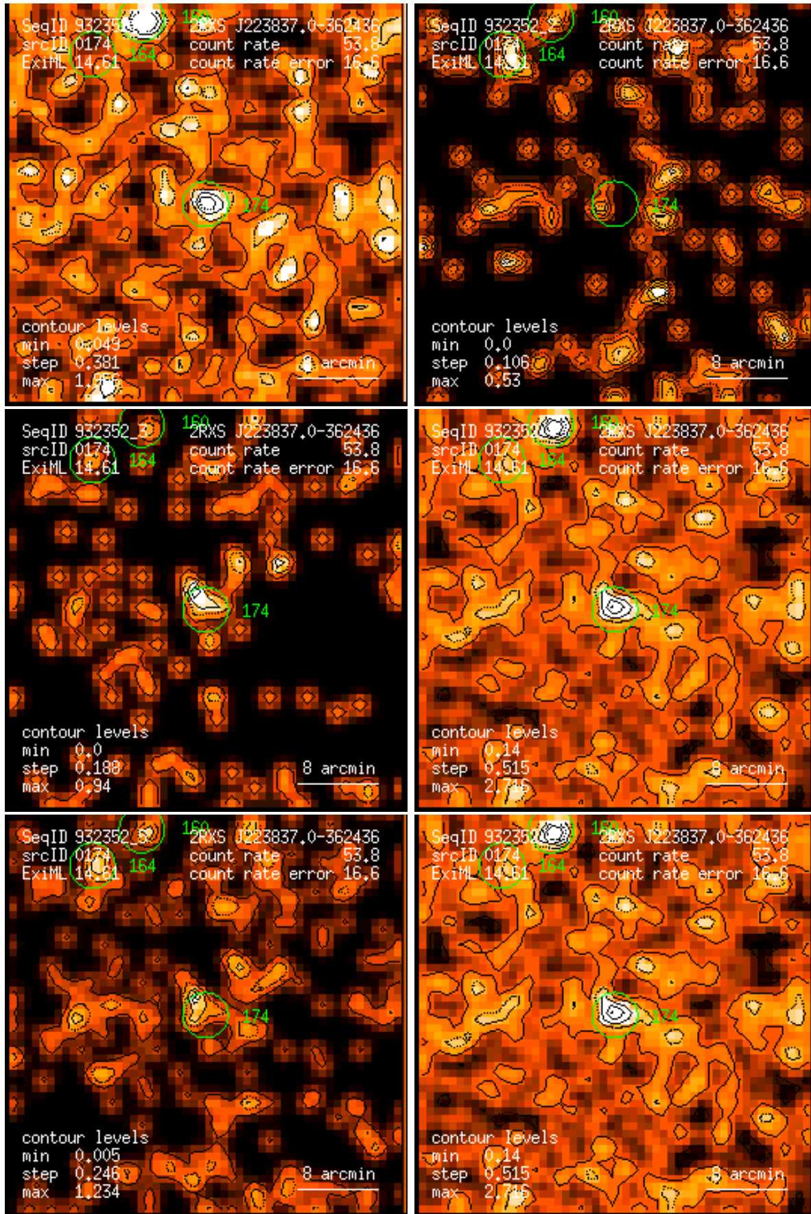
Figure 174: RASS 932352: detection 0174: band rate images, Gaussian filter: (1) PSPC channels 11 – 41, (2) 52 – 90, (3) 91 – 201, (4) 11 – 235, (5) 52 – 201, (6) 11 – 201. Broad band rates in counts/ks. Band rate contour levels in counts/ks/arcmin 2 .
