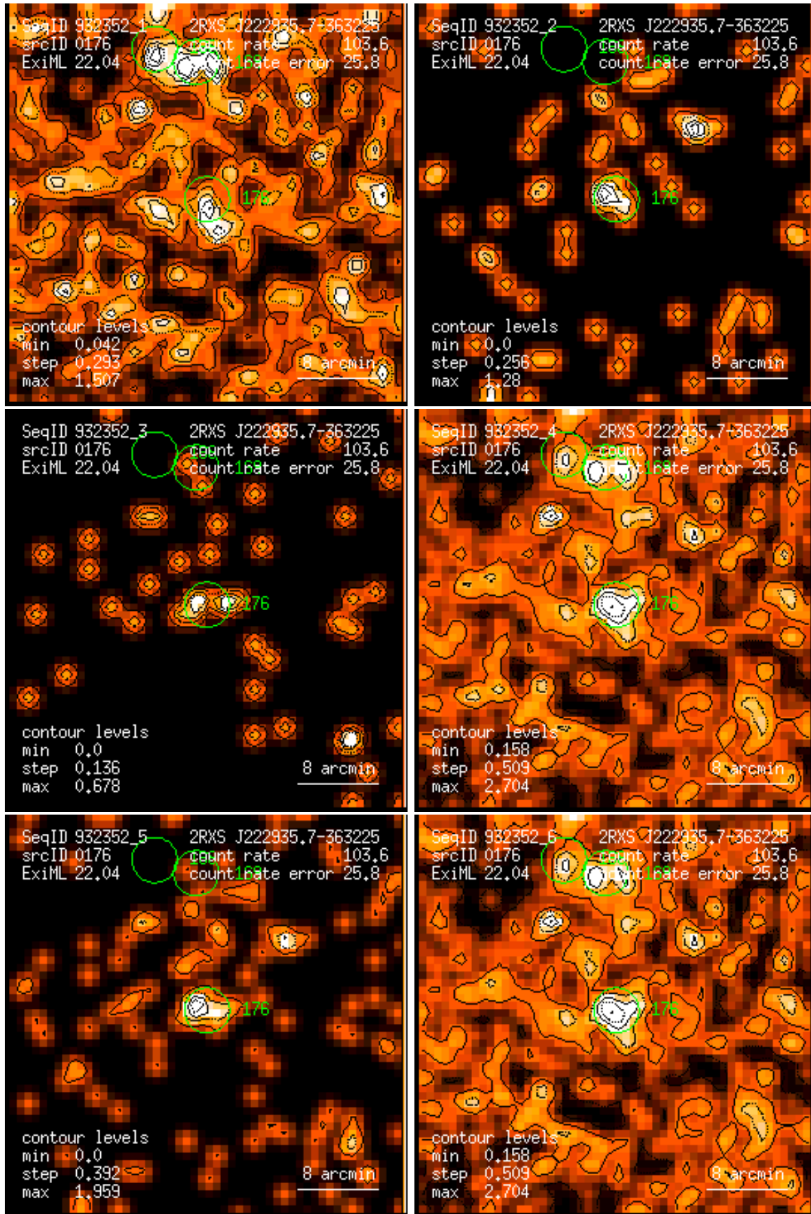
Figure 176: RASS 932352: detection 0176: band rate images, Gaussian filter: (1) PSPC channels 11 – 41, (2) 52 – 90, (3) 91 – 201, (4) 11 – 235, (5) 52 – 201, (6) 11 – 201. Broad band rates in counts/ks. Band rate contour levels in counts/ks/arcmin 2 .
