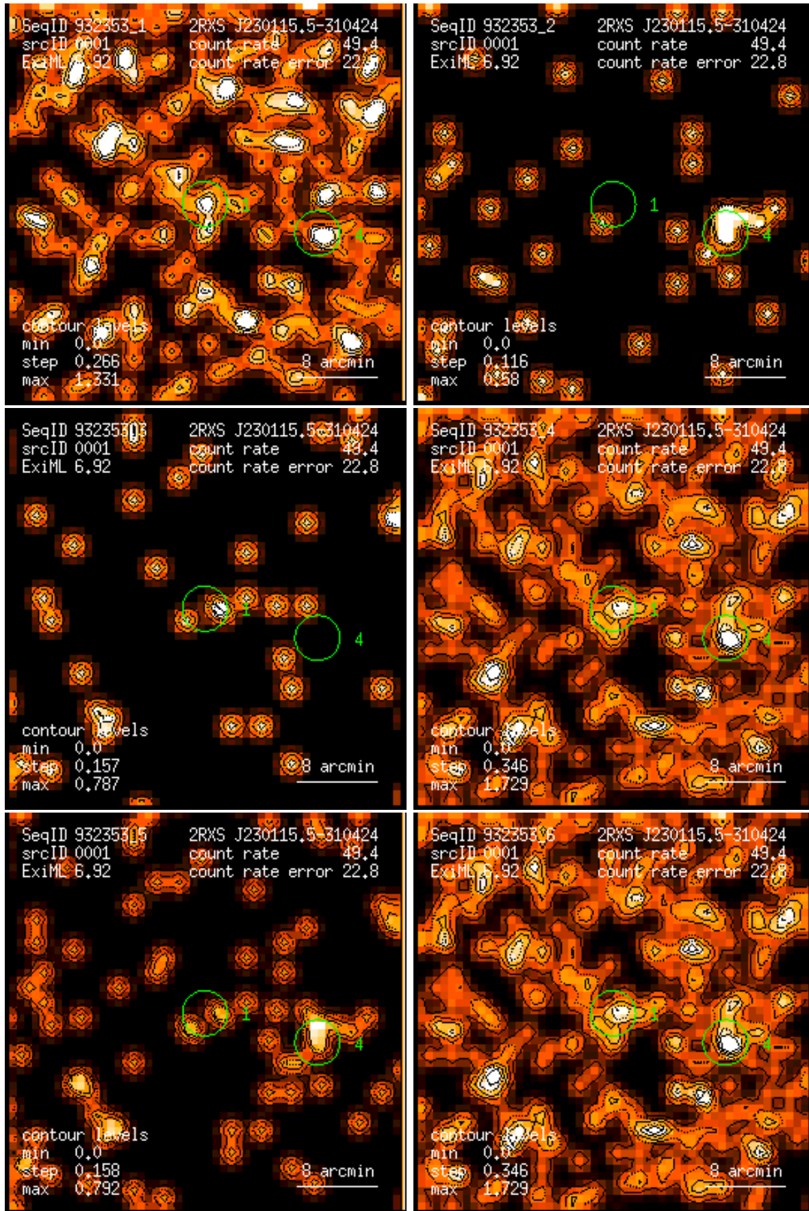
Figure 1: RASS 932353: detection 0001: band rate images, Gaussian filter: (1) PSPC channels 11 – 41, (2) 52 – 90, (3) 91 – 201, (4) 11 – 235, (5) 52 – 201, (6) 11 – 201. Broad band rates in counts/ks. Band rate contour levels in counts/ks/arcmin 2 .
