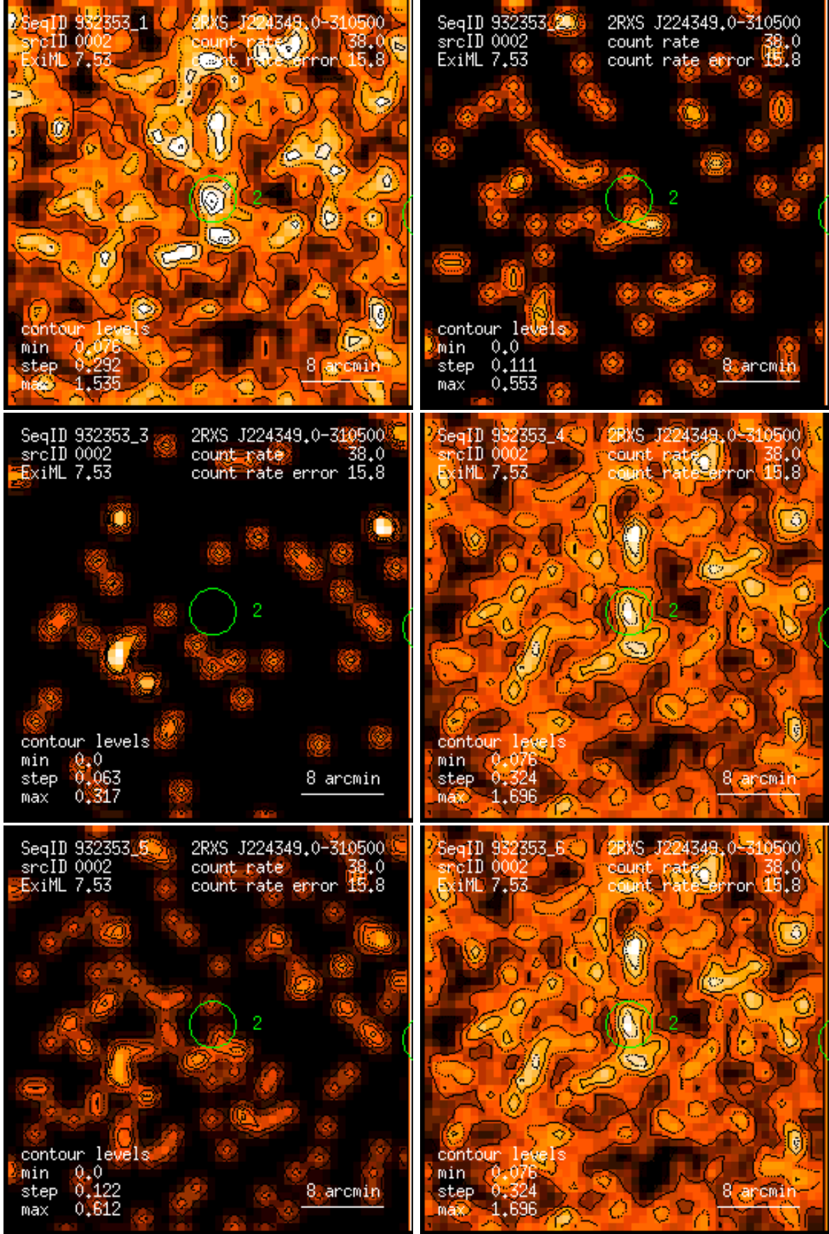
Figure 2: RASS 932353: detection 0002: band rate images, Gaussian filter: (1) PSPC channels 11 – 41, (2) 52 – 90, (3) 91 – 201, (4) 11 – 235, (5) 52 – 201, (6) 11 – 201. Broad band rates in counts/ks. Band rate contour levels in counts/ks/arcmin 2 .
