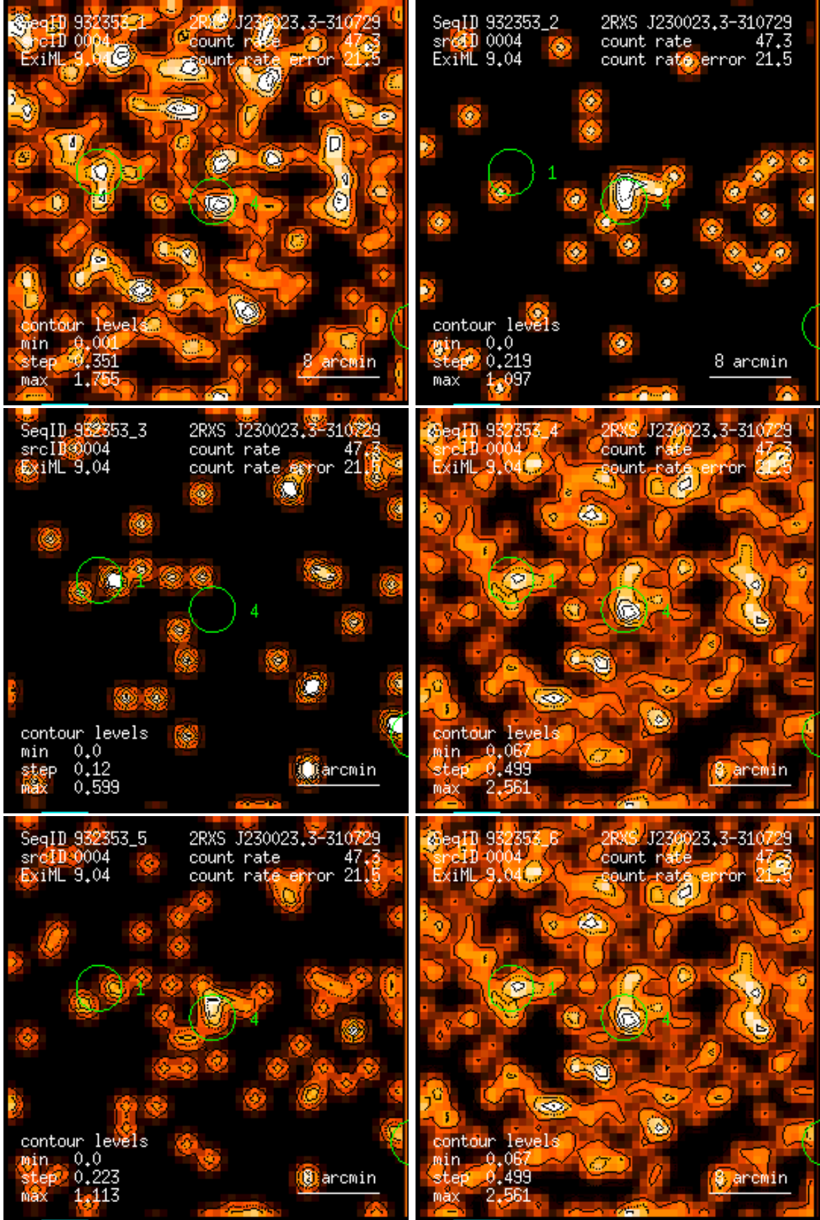
Figure 4: RASS 932353: detection 0004: band rate images, Gaussian filter: (1) PSPC channels 11 – 41, (2) 52 – 90, (3) 91 – 201, (4) 11 – 235, (5) 52 – 201, (6) 11 – 201. Broad band rates in counts/ks. Band rate contour levels in counts/ks/arcmin 2 .
