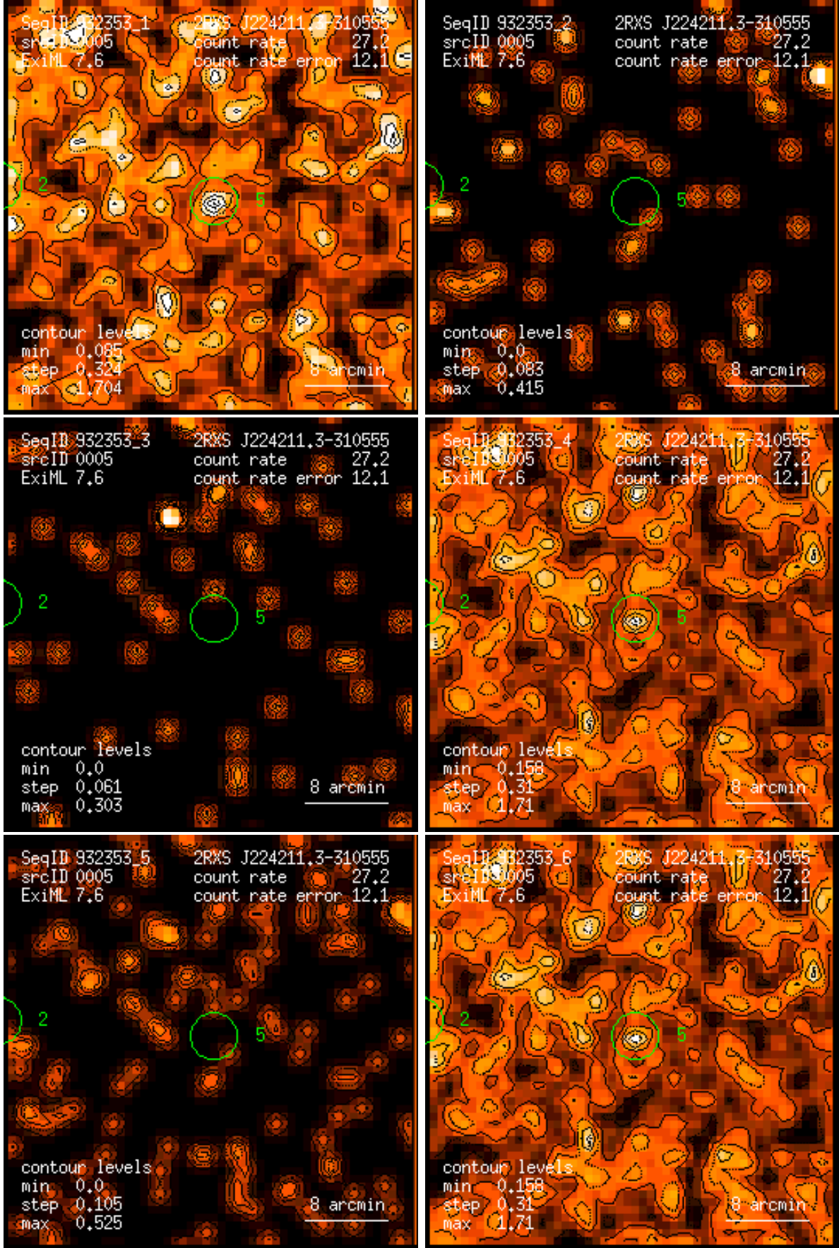
Figure 5: RASS 932353: detection 0005: band rate images, Gaussian filter: (1) PSPC channels 11 – 41, (2) 52 – 90, (3) 91 – 201, (4) 11 – 235, (5) 52 – 201, (6) 11 – 201. Broad band rates in counts/ks. Band rate contour levels in counts/ks/arcmin 2 .
