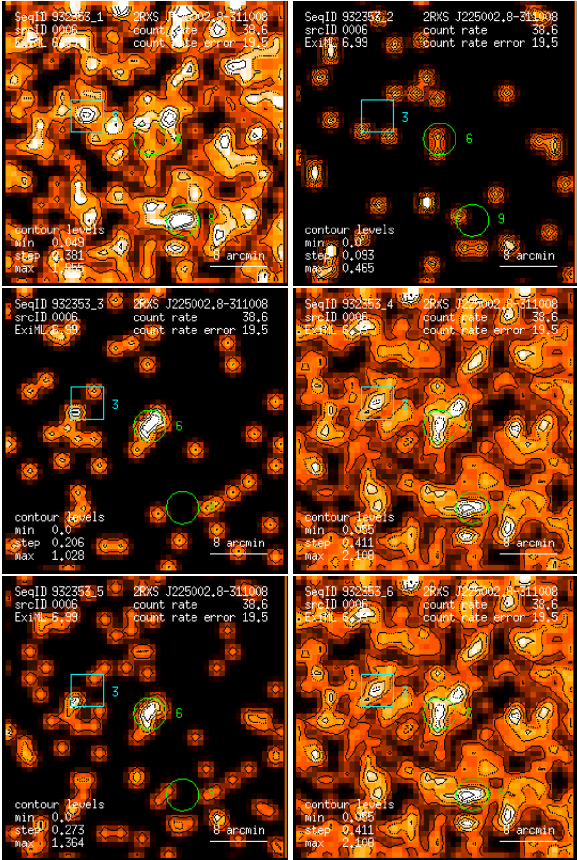
Figure 6: RASS 932353: detection 0006: band rate images, Gaussian filter: (1) PSPC channels 11 – 41, (2) 52 – 90, (3) 91 – 201, (4) 11 – 235, (5) 52 – 201, (6) 11 – 201. Broad band rates in counts/ks. Band rate contour levels in counts/ks/arcmin 2 .
