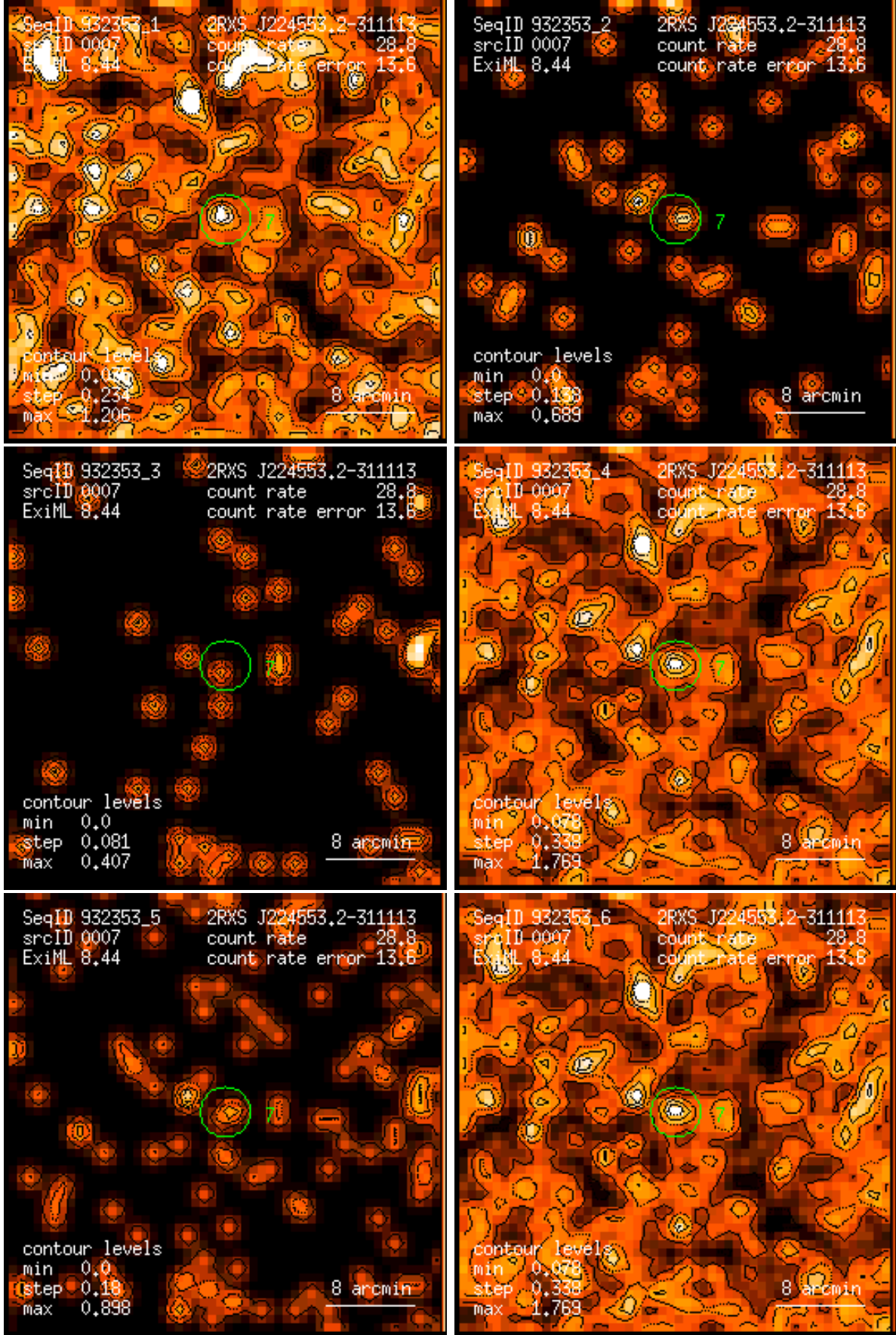
Figure 7: RASS 932353: detection 0007: band rate images, Gaussian filter: (1) PSPC channels 11 – 41, (2) 52 – 90, (3) 91 – 201, (4) 11 – 235, (5) 52 – 201, (6) 11 – 201. Broad band rates in counts/ks. Band rate contour levels in counts/ks/arcmin 2 .
