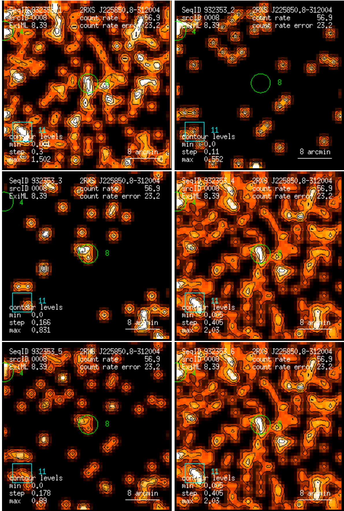
Figure 8: RASS 932353: detection 0008: band rate images, Gaussian filter: (1) PSPC channels 11 – 41, (2) 52 – 90, (3) 91 – 201, (4) 11 – 235, (5) 52 – 201, (6) 11 – 201. Broad band rates in counts/ks. Band rate contour levels in counts/ks/arcmin 2 .
