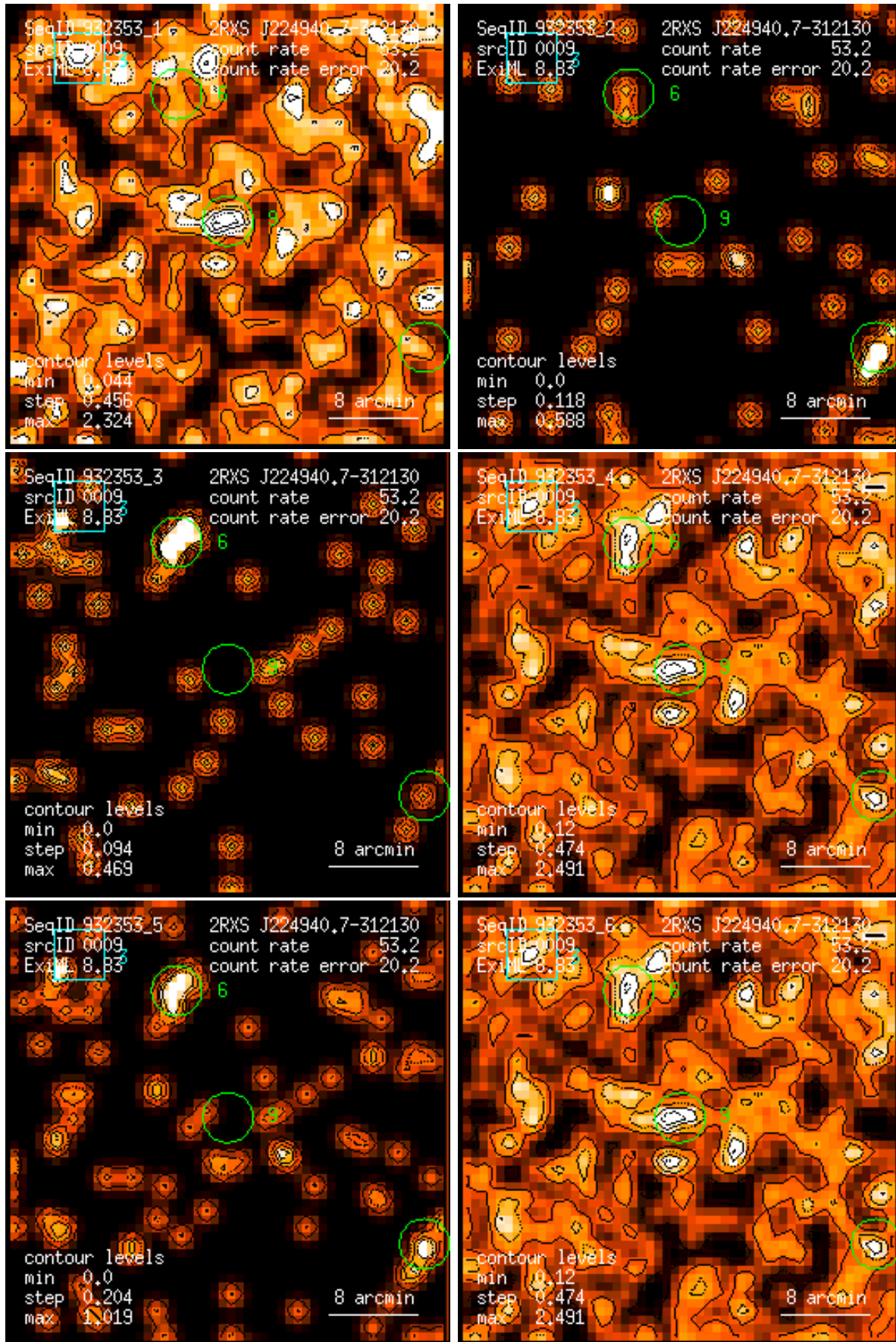
Figure 9: RASS 932353: detection 0009: band rate images, Gaussian filter: (1) PSPC channels 11 – 41, (2) 52 – 90, (3) 91 – 201, (4) 11 – 235, (5) 52 – 201, (6) 11 – 201. Broad band rates in counts/ks. Band rate contour levels in counts/ks/arcmin 2 .
