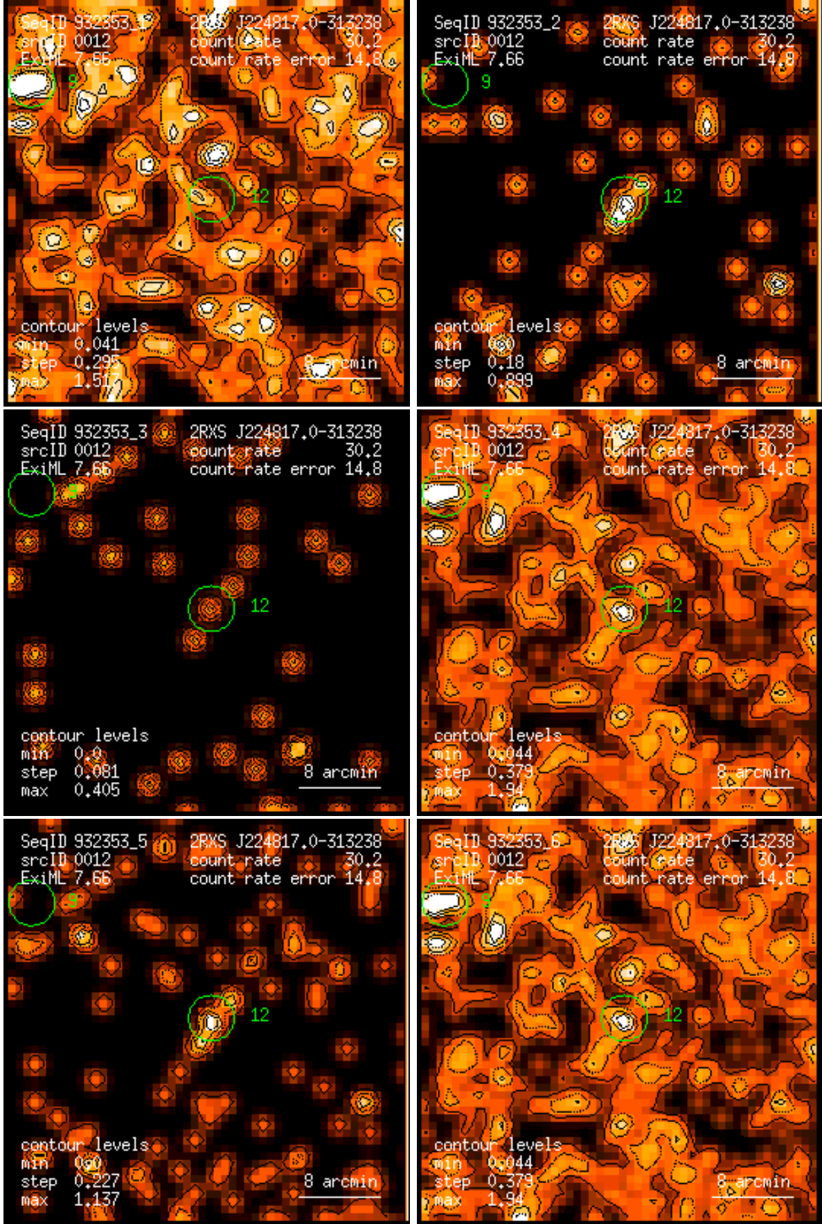
Figure 12: RASS 932353: detection 0012: band rate images, Gaussian filter: (1) PSPC channels 11 – 41, (2) 52 – 90, (3) 91 – 201, (4) 11 – 235, (5) 52 – 201, (6) 11 – 201. Broad band rates in counts/ks. Band rate contour levels in counts/ks/arcmin 2 .
